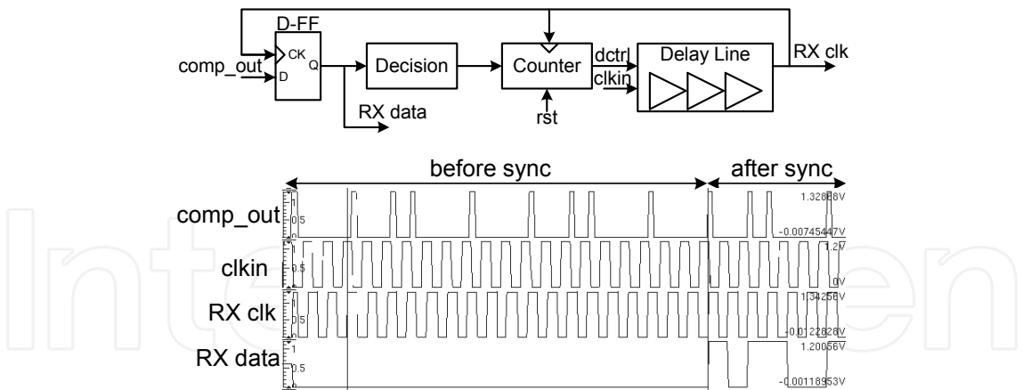
Fig. 19. Clock and data synchronization
