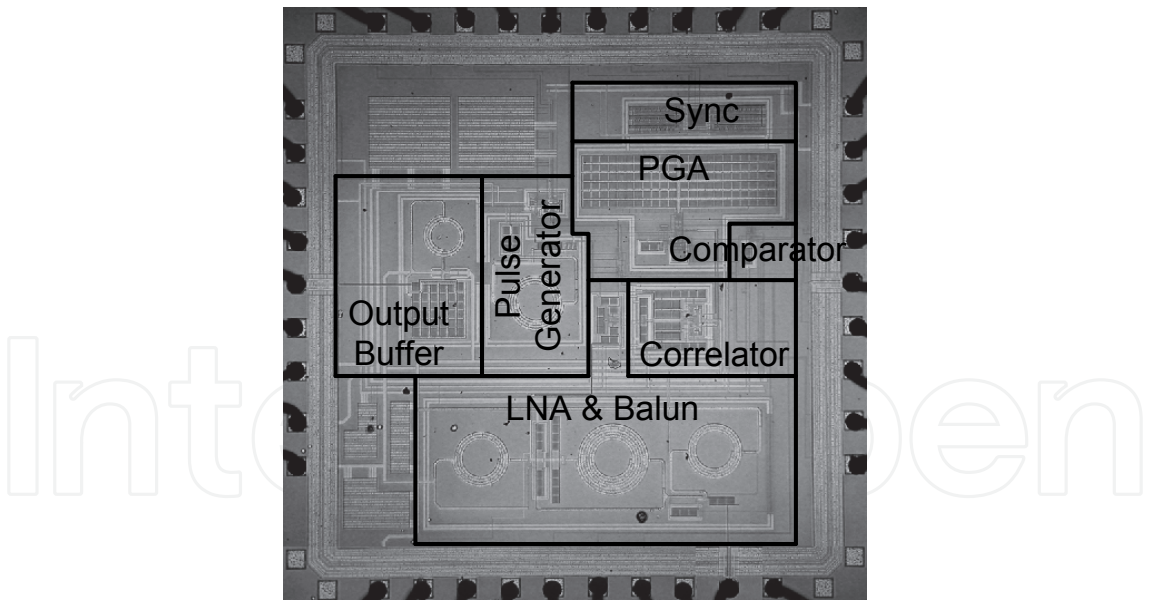
Fig. 20. Microphotograph of IR-UWB transceiver
