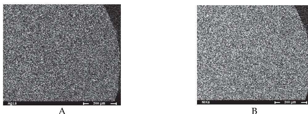
Fig. 21. The distribution of Ag (A) and Ni (B) particles on the surface of the granule of the \text{SiO}_2 -10%AgNi(1:4) composite
