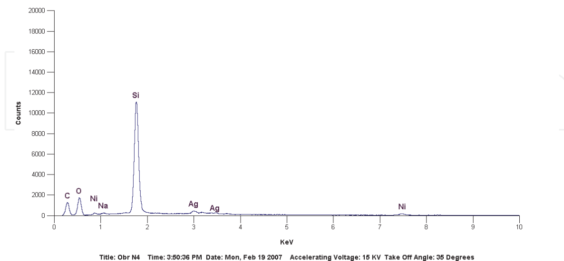
Fig. 20. The X-ray diffraction spectrum of the \text{SiO}_2 -10%AgNi(1:4) composite
