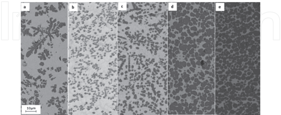
Fig. 17. Developed TiC morphologies using laser condition A for compositions of: a) 745 b) 755 c) 655 d) 555 e) 155
