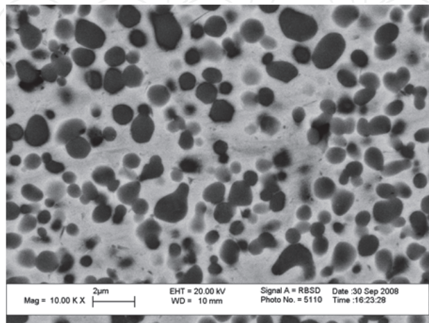
Fig. 4. BSE image-distributed black particles in matrix of a one layer clad (sample 23)
