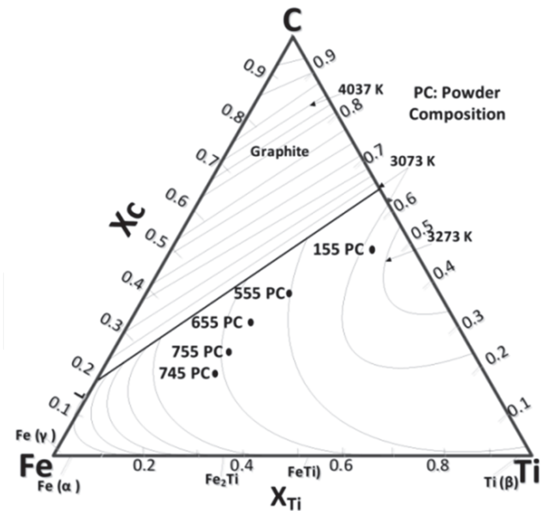
Fig. 9. Liquid projection
