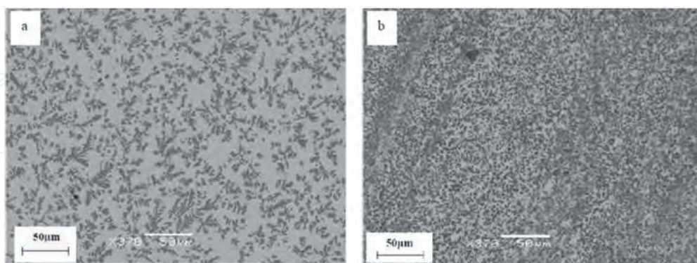
Fig. 16. TiC morphology of samples a) D1 and b) D2
