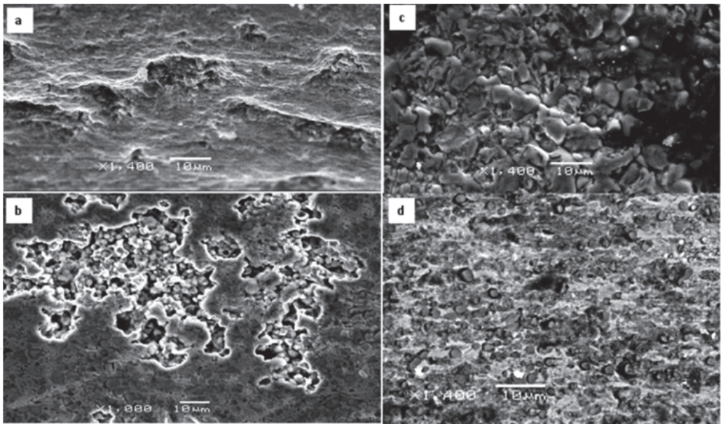
Fig. 21. (a) Plastic deformations in worn surface of 745A (b) Pulling out of carbides in worn surface of 755A (c) Worn matrix and remaining TiC particles in sample 155A (d) Worn matrix and remaining TiC particles in sample 755B
