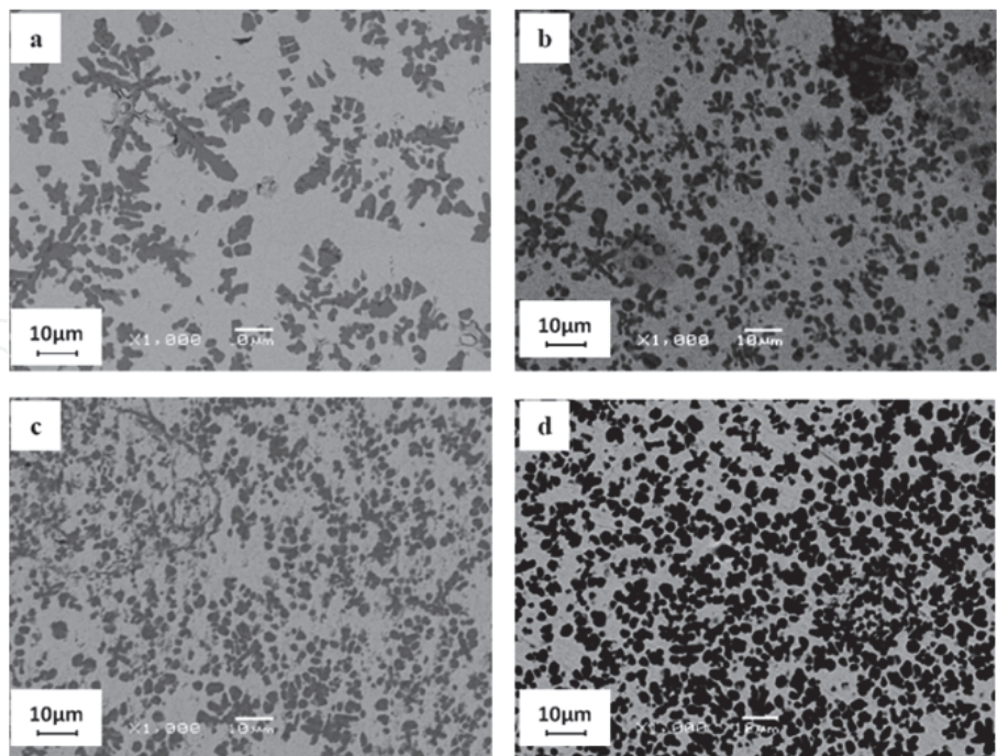
Fig. 14. a) Sample B3 b) sample B4 c) sample B5 d) sample B6
