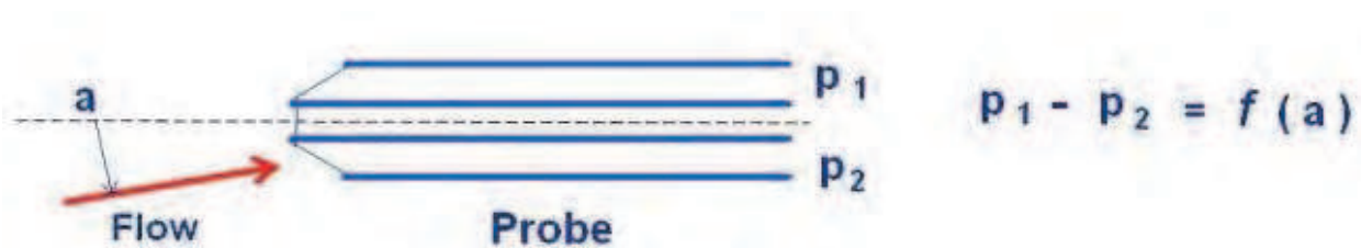
Fig. 3. Vertical cut of three tubes showing the leading edges and the angle determination concept
