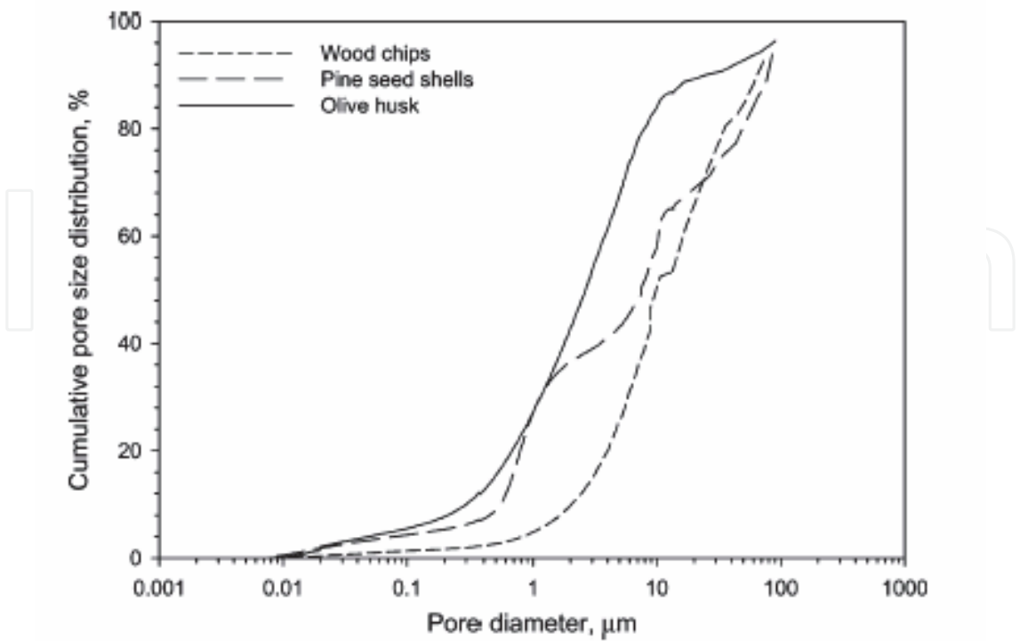
Fig. 7. Cumulative pore size distribution of three biomass chars from Hg porosimetry
