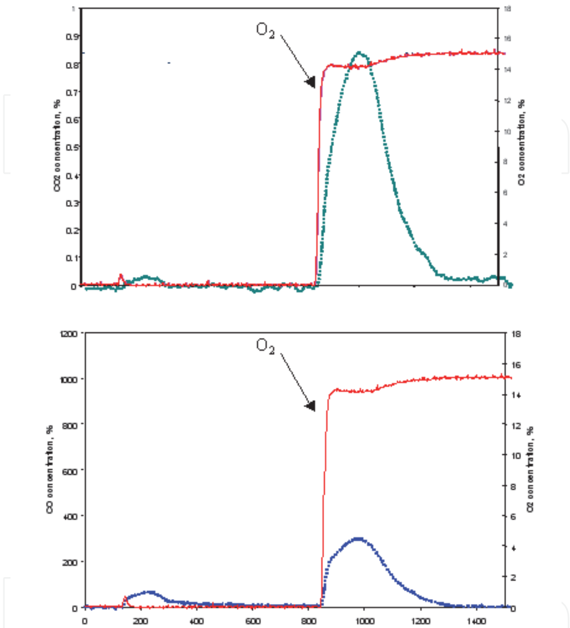
Fig. 17. Profiles of O 2 CO and CO 2 released during an experiment of TRCCI at 600°C in the fluidized bed reactor for a residue of the oil industry
