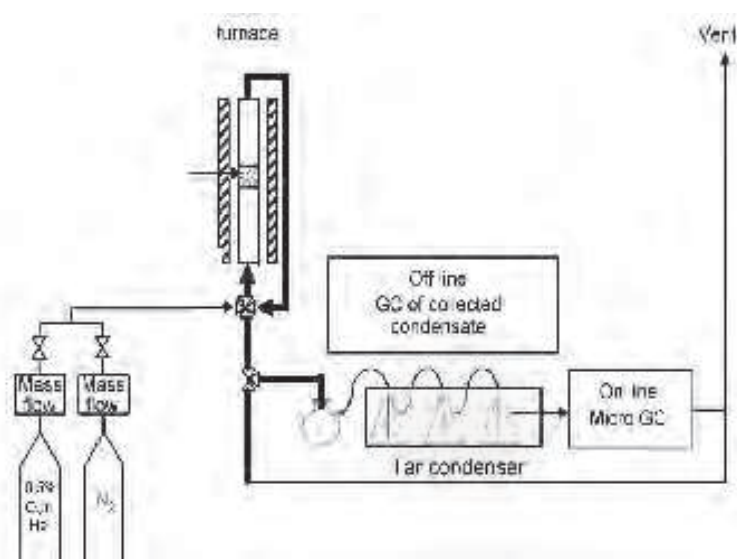
Fig. 4. Lab scale pyrolysis reactor.
