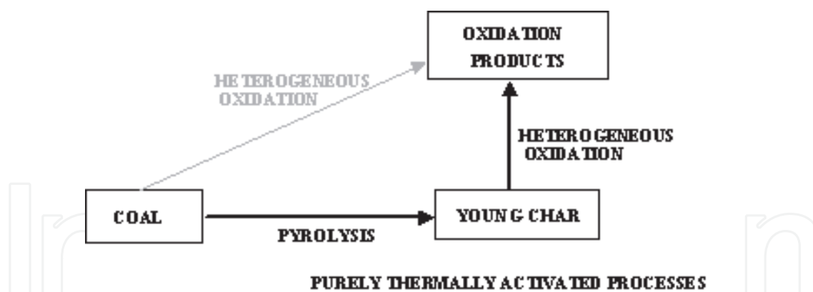
Fig. 2. B Reaction path of pyrolysis-char combustion
