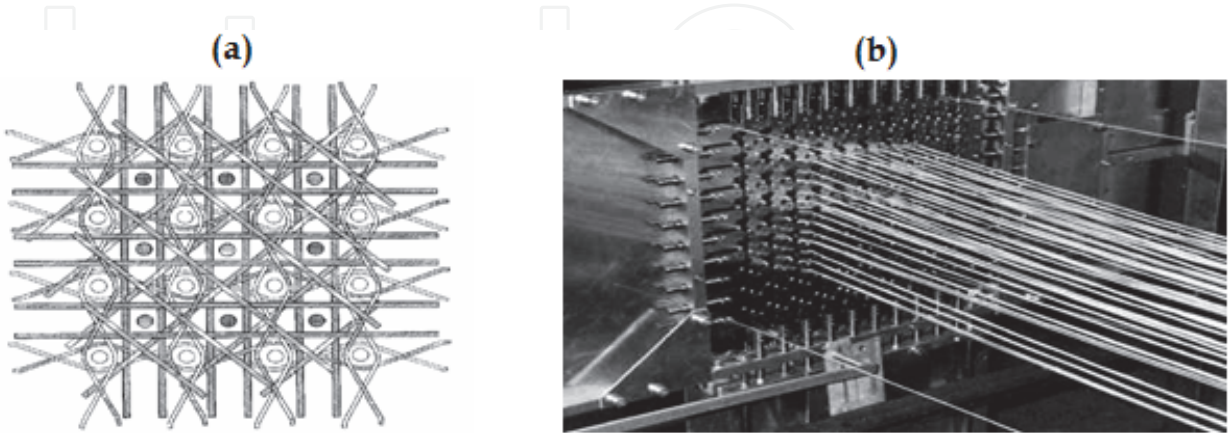
Fig. 18. The fabric (a) and specially designed loom to fabricate the multiaxis 3D fabric (b) (Khokar, 2002b).
