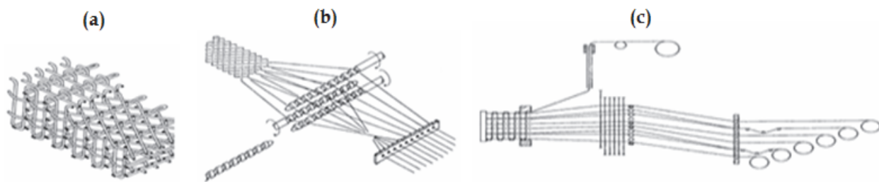
Fig. 19. The multiaxis 3D woven fabric (a), indexing mechanism for \pm bias (b) and loom (c) (Anahara and Yasui, 1992).
