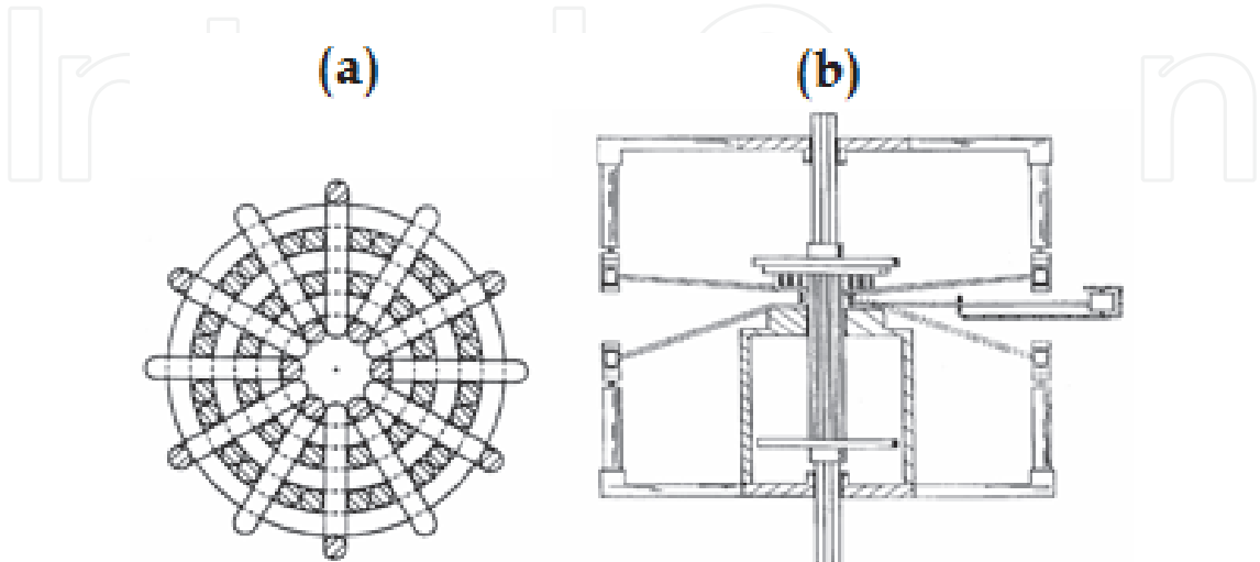
Fig. 11. 3D circular woven perform (a) and weaving loom schematic (b) (Yasui et al., 1992).
