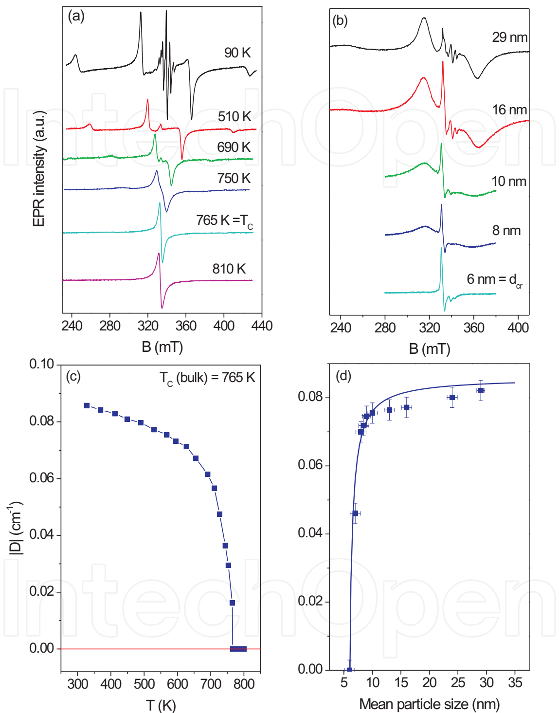
Fig. 5. (a,b) - X-band EPR spectra of \text{Cr}^{3+} -doped \text{PbTiO}_3 . (a) - temperature dependent EPR spectra of bulk \text{Cr}^{3+}:\text{PbTiO}_3 . (b) - size-dependent EPR spectra of \text{Cr}^{3+}:\text{PbTiO}_3 nano-powders measured at ambient temperature. (c,d) - phase transition monitored via the axial fine-structure parameter D .
