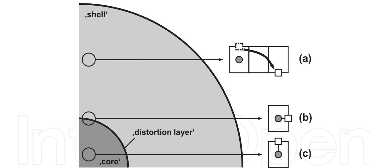
Fig. 8. Schematic illustration of the 'core-shell structure' for \text{Fe}^{3+} -doped \text{PbTiO}_3 ferroelectric nano-particles. (a) - 'isolated' \text{Fe}_{\text{Ti}}' and \text{V}_{\text{O}}'' defects at the paraelectric surface. (b) - (\text{Fe}_{\text{Ti}}' - \text{V}_{\text{O}}'')^\bullet defect complexes of rhombic site symmetry at interface layer. (c) - (\text{Fe}_{\text{Ti}}' - \text{V}_{\text{O}}'')_{||} defect dipoles at the ferroelectric core. The corresponding unit cells are illustrated by rectangles, the \text{Fe}^{3+} -functional centers by a gray circle and the oxygen vacancies by open squares.
