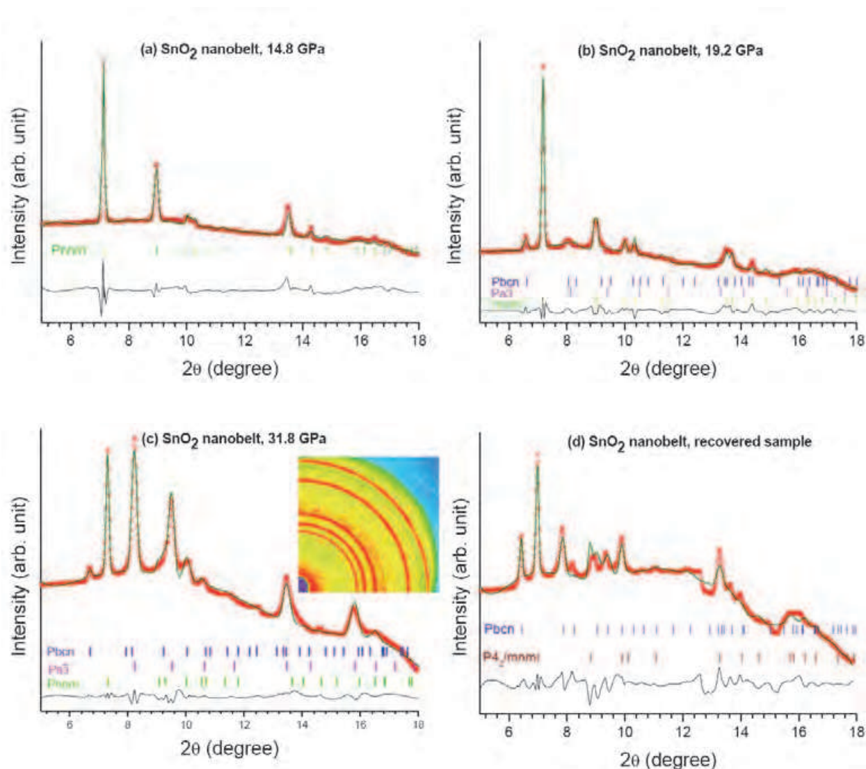
Fig. 6. Rietveld refinement of X-ray diffraction patterns of \text{SnO}_2 nanobelts at 14.8 GPa (a), 19.2 GPa (b), 31.8 GPa (c) and from recovered sample (d). The inset in (c) shows the original 2D Debye-Scherrer patterns with one quadrant. The red cross is experimental X-ray intensity whereas the green solid line is the calculated diffraction pattern based on refinement with the black curve at the bottom showing the difference between the calculated and observed intensities. The vertical bars with different colors indicate the characteristic reflections of different phases labeled in the front.
