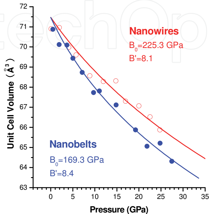
Fig. 9. Pressure-volume relations for \text{SnO}_2 nanowires (open circles) and nanobelts (solid circles). The solid lines are fittings using 3 rd order Birch equation of state (see text).
