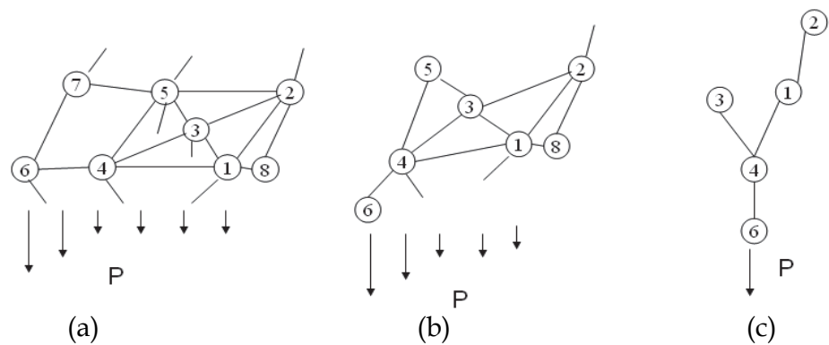
Fig. 20. Atomic deformation of TiO 2 type nanowires, showing a concentration of bond forces at the surface.
