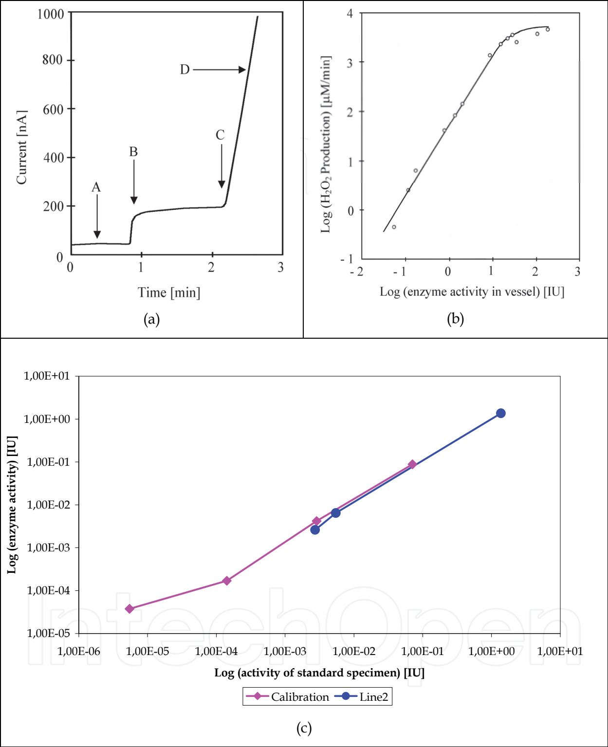
Fig. 12. a) Schematic view of enzyme activity measurement; A) addition of glucosse concentration in vessel c_{\text{vessel}} = 500 \text{ mM} ; B) addition of H 2 O 2 for calibration c_{\text{vessel}} = 20.2 \text{ }\mu\text{M} ; C) injection of GOx solution of unknown activity; D) H 2 O 2 production (478 \mu\text{M}/\text{min} ). b) Calibration curve for enzyme activity measurement using MFS (Krejci et al., 2008). c) Calibration curve for enzyme activity measurement using RDE.
