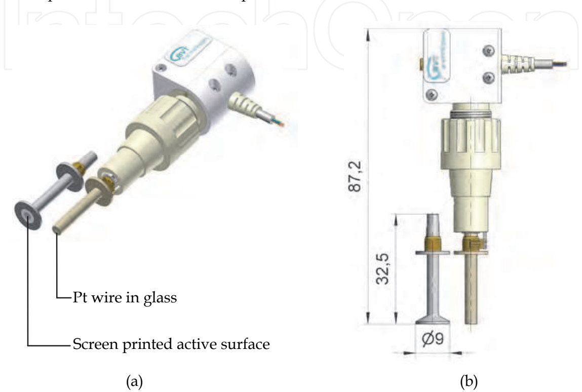
Fig. 7. a, b) Mini-rotated disc electrode The principle of RDE can be enhanced to move complicated hydro-dynamical arrangement. It can be used for elimination of cross talk of array of electrodes (Dock et al., 2005; Sajdlová, 2010). The comparison of conversion efficiencies for typical parameters used in measurement in experimental part are summarized in tab. 4. The parameters are: diameter of jet nozzle a = 0.5 \text{ mm} ; radius of electrode R = 1 \text{ mm} ; height of channel h = 0.3 \text{ mm} ; width of channel b = 1 \text{ mm} ; length of electrode l = 2 \text{ mm} ; diffusion coefficient D = 10^{-9} \text{ m}^2 \text{ s}^{-1} ; kinematics' viscosity of water \nu = 10^{-6} \text{ m}^2 \text{ s}^{-1} ; angular speed of RDE \omega = 60 \text{ s}^{-1}
