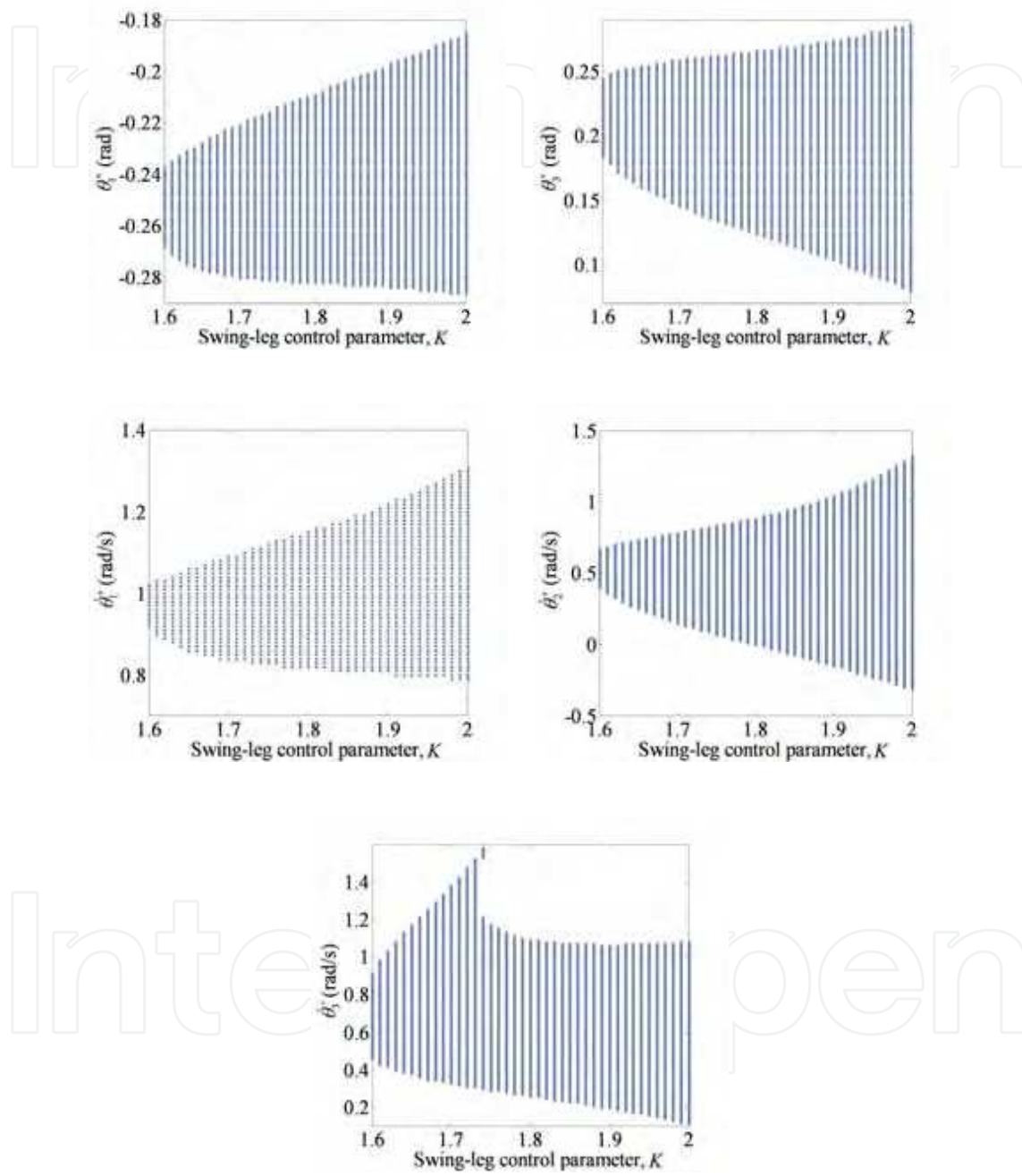
Figure 4. Stable range as a function of the swing-leg control parameter K where \theta_s^d = 0.2
