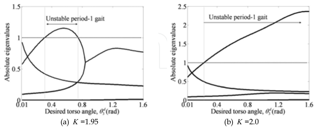
Figure 3. Absolute eigenvalues versus desired torso angle
