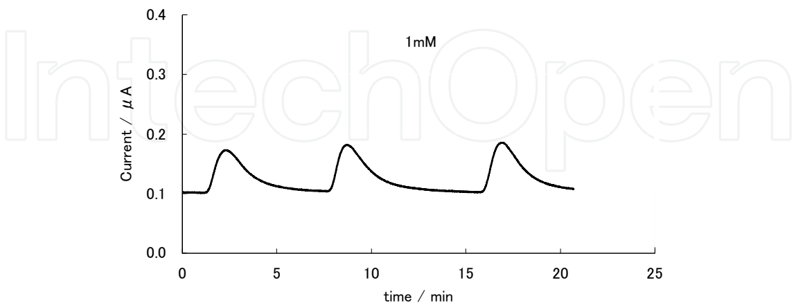
Fig. 9. Diagram of amperometric response obtained with the sensor system for successive injections of 2,4-D standard solution (pH 6.5; H = 3\text{ mm} ; flow rate 1.0\text{ mL/min} ).
