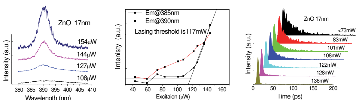
Fig. 5. The ultrafast light emission from ZnO nanoparticles.
