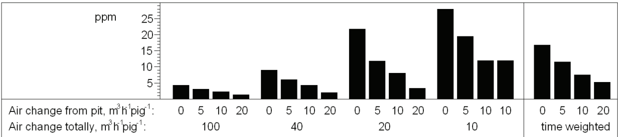
Fig. 9. Ammonia concentration in room exhaust at different pit ventilation and entire unit ventilation. Time weighted values, shown to the right in the graph, assumes total air change of 100 m 3 h -1 Pig -1 in 10 percent of time, and 40, 20 and 10 m 3 h -1 Pig -1 in 30 percent of time each.
