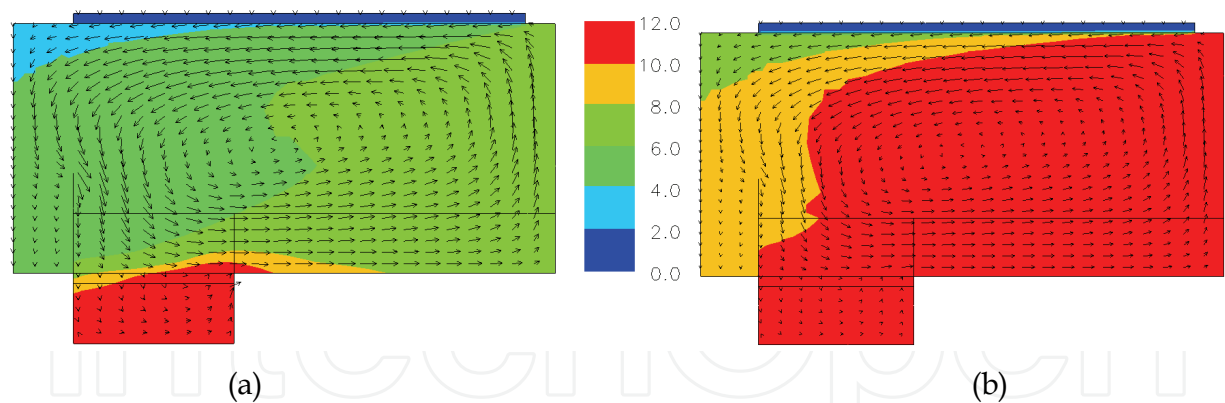
Fig. 8. Simulated airflow and ammonia distributions (ppm) at total ventilation of 40 m 3 h -1 Pig -1 , (a) with pit ventilation of 10 m 3 h -1 Pig -1 , and (b) without pit ventilation.
