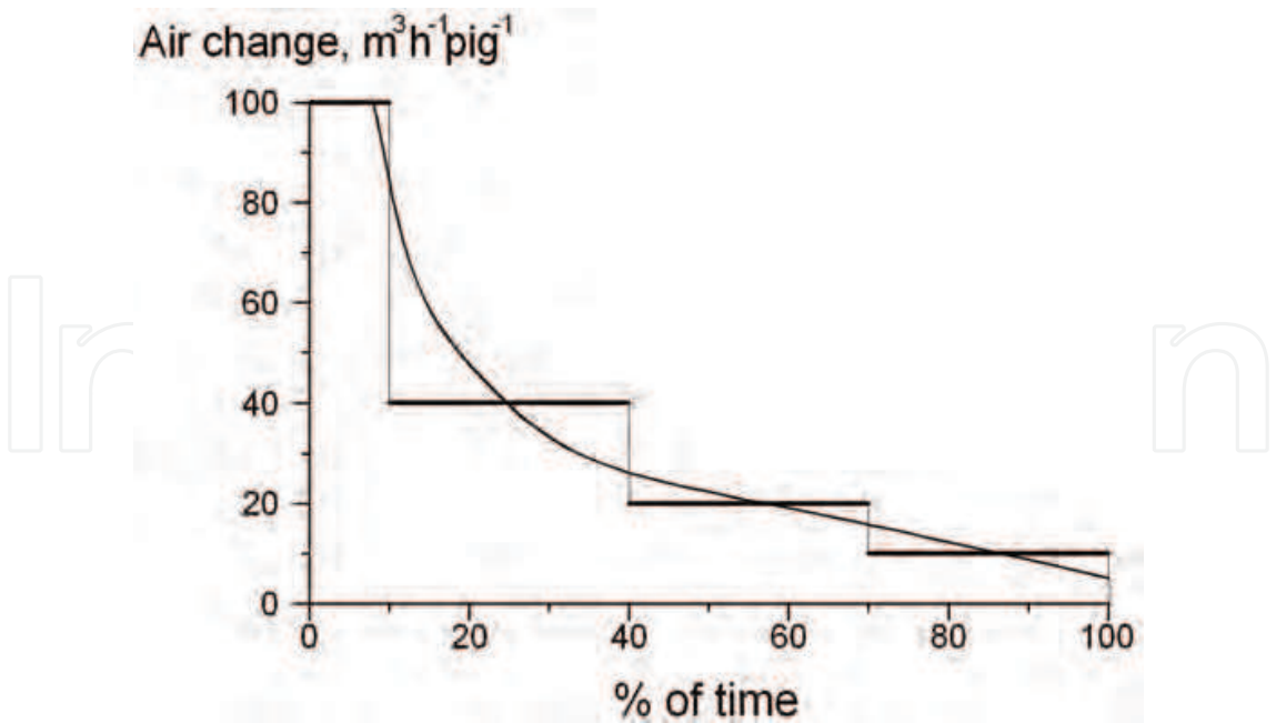
Fig. 4. Expected distribution of ventilation levels in a growing pig unit under Danish conditions (smooth curve), and four representative levels of ventilation (step curve) used in modelling of ammonia release and emission.
