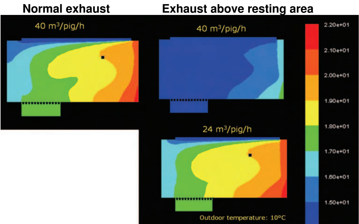
Fig. 13. CFD prediction of temperature distributions (°C) in a pig pen at different exhaust locations and air changes.
