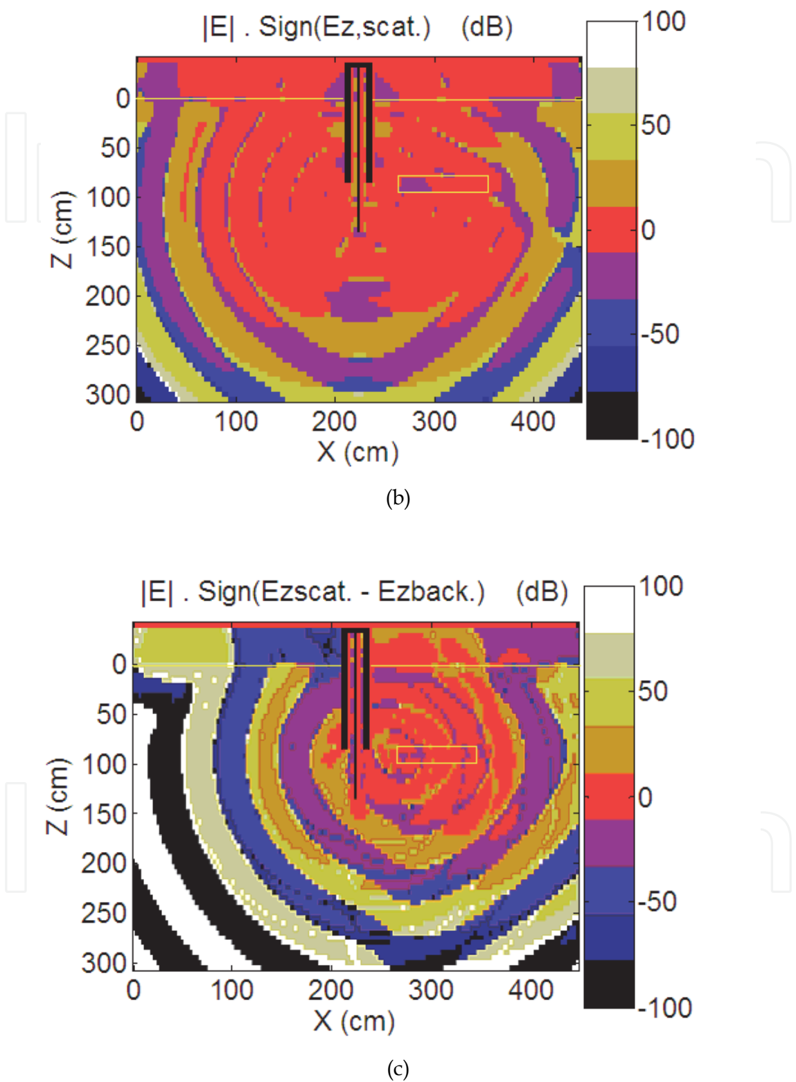
Fig. 9. Electric field, [Sign(E_{z,Total} - E_{z,Incident})] \times 20 \log_{10}(|E| \text{ or } |E_x \vec{i} + E_z \vec{k}|) , on the depth slice (XZ-plane) at time t = 90 nsec (the extent of the DNAPL pool and soil-air interface are marked in yellow): a) Incident image, b) Total image, and c) Scattered image.
