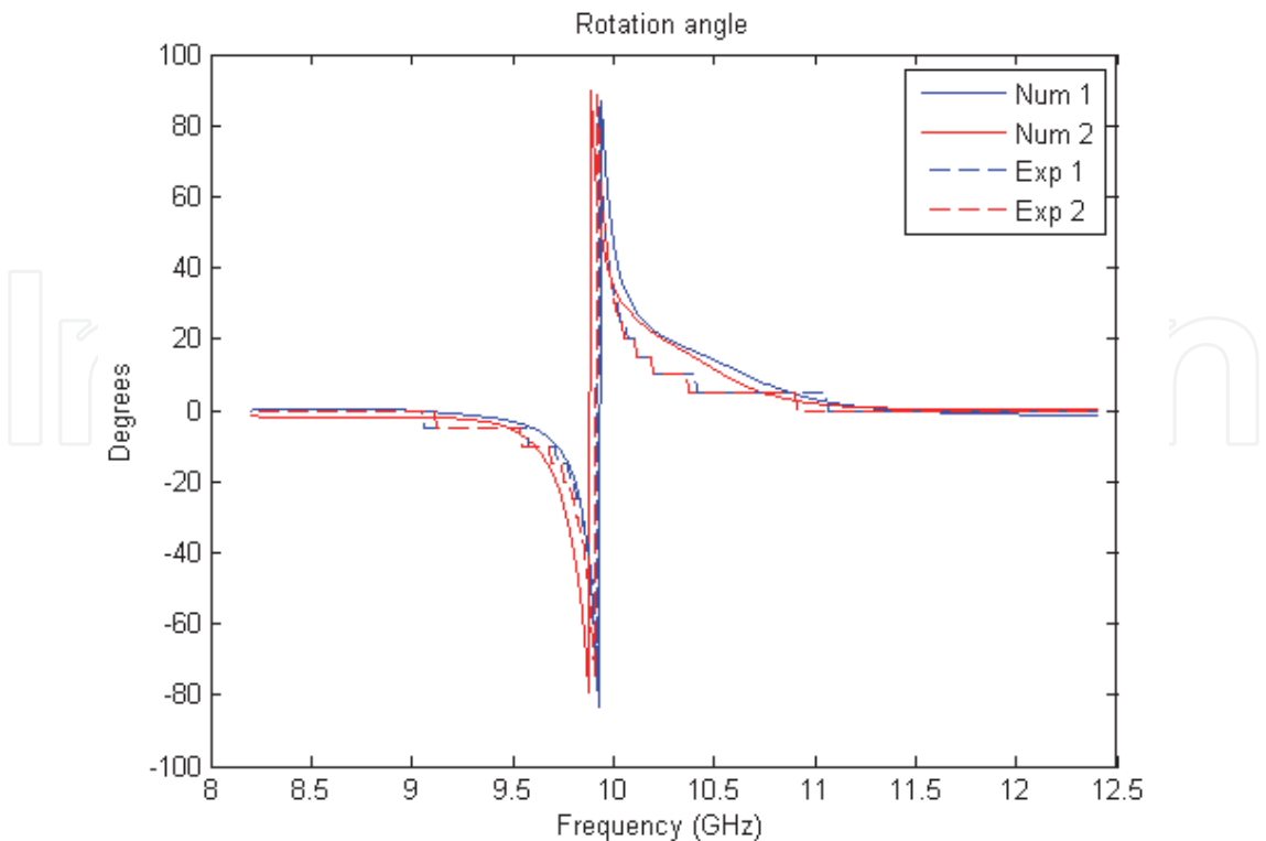
Fig. 13. Rotation of the polarization angle for a plane wave normally incident over a quasi-planar periodic array of right-handed cranks as shown in Figs. 3 and 6: numerical (Num) and experimental (Exp) results. 1 and 2 represent the two possible directions of the propagation wave (incident from front and back side, respectively).
