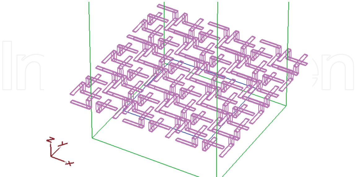
Fig. 14. MEFiSTo™ model of a condensed array of cranks. Each crank is composed by two arms, 3mm long, one in each side of the board (1.5 mm of thickness), plus a via connecting both.
