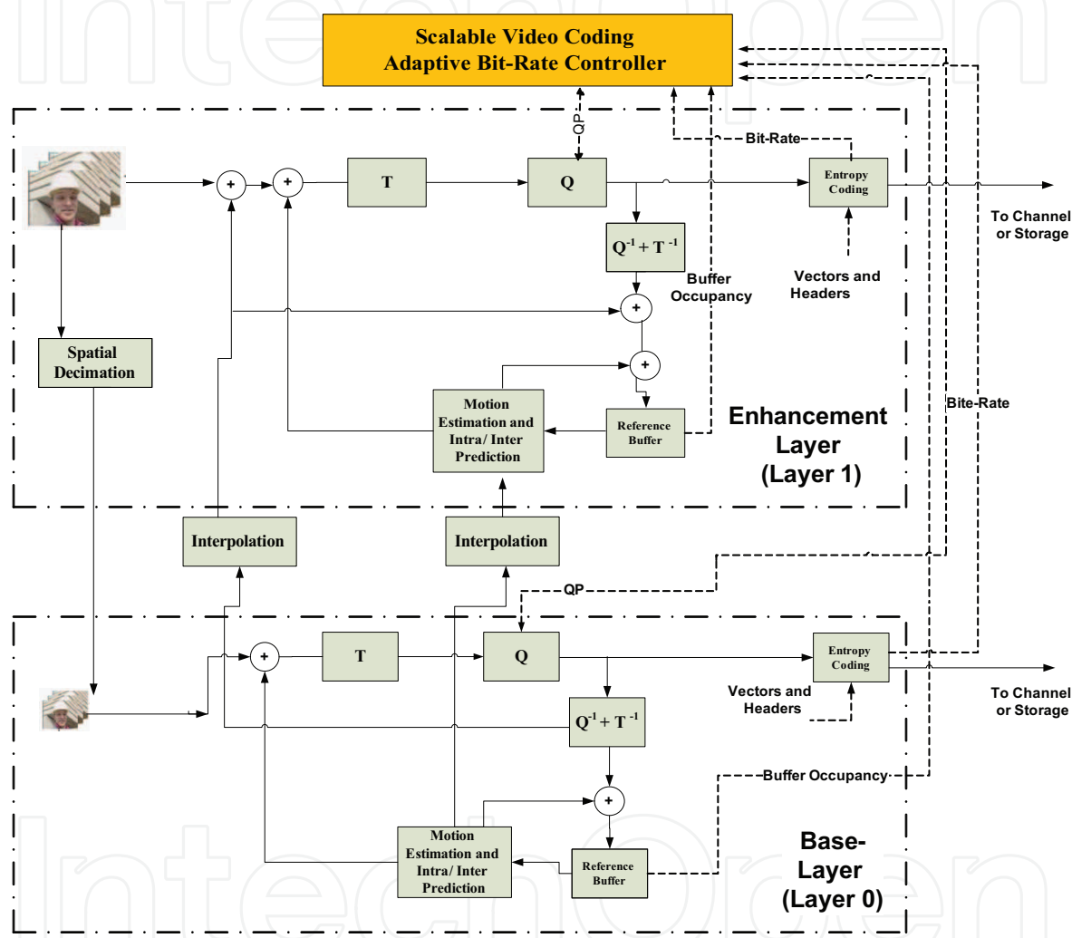
Fig. 7. The system for performing the presented adaptive spatial bit-rate control for the Scalable Video Coding (for simplicity, only two layers – Layer 0 and Layer 1 - are presented). The optimal buffer control approach is related to the following optimal bit allocation formulation,
