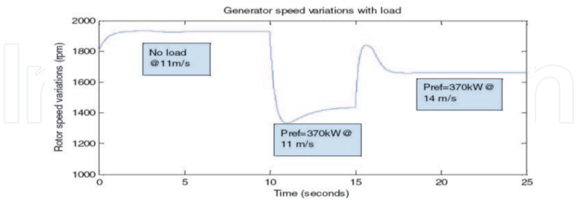
Fig. 18. Rotor speed variations with load
