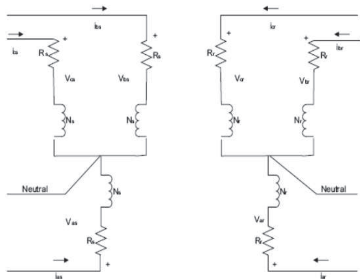
Fig. 6. Two-pole, 3-phase, wye connected symmetrical induction machine.
