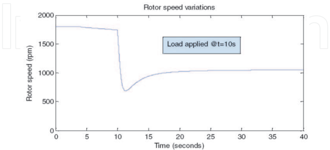
Fig. 14. Generator speed (For failed excitation case)
