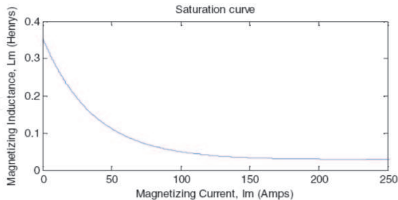
Fig. 9. Variation of magnetizing inductance with magnetizing current.
