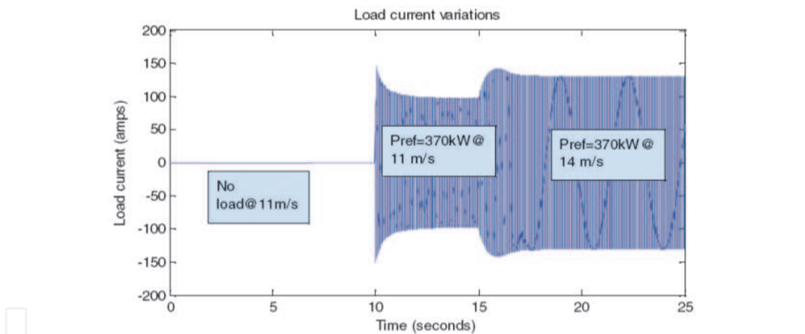
Fig. 20. Load current variations with load.
