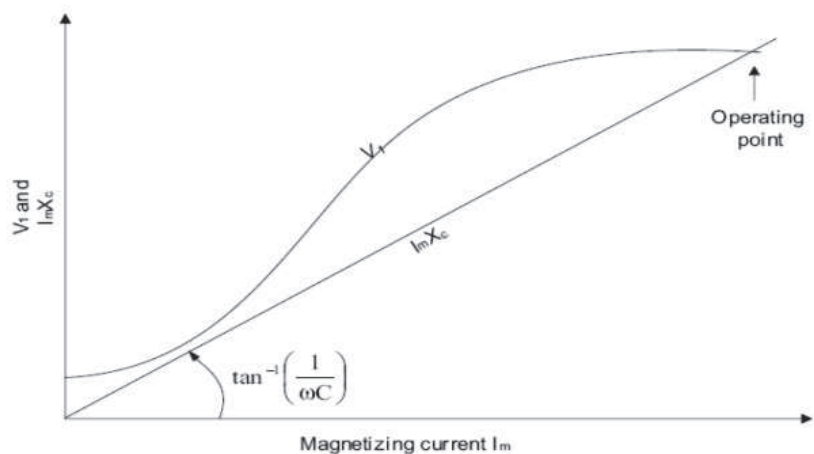
Fig. 3. Determination of stable operation of self-excited induction generator.
