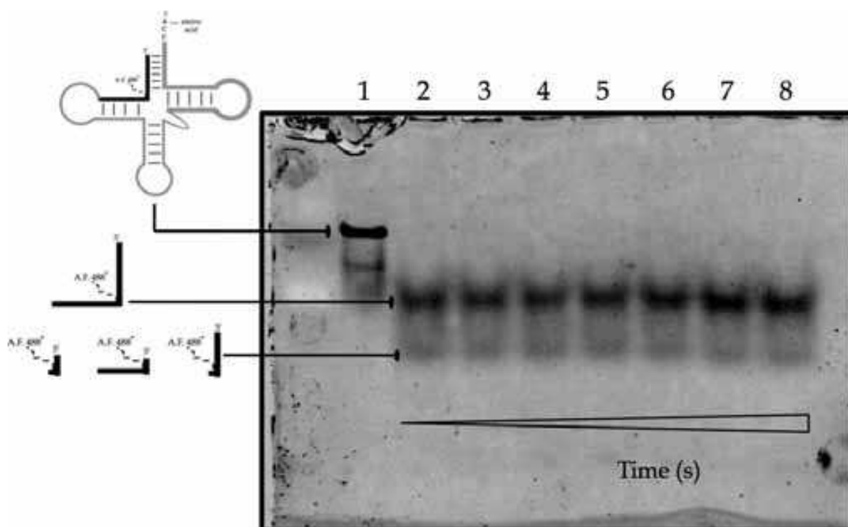
Fig. 18. Polyacrylamide gel analysis of the hydrolysis of labelled ValRNA Val-488 with the RNase cocktail – RNase A/ T1. Lane 1 corresponds to 5.0 \mu M ValRNA Val-488 in the absence of RNases. Lanes 2 – 8 correspond to individual ValRNA Val-488 (5.0 \mu M) samples incubated with RNase A/ T1 cocktail (1.25 Units A & 50 Units T1) for 5, 10, 15, 20, 25, 30 and 60 seconds, respectively. Each reaction was quenched with unfractionated yeast total tRNA (1.0 mg/ mL). Gel conditions: 15% tris boric acid gel, 1X TBE running buffer (90 mM Trisma, 90 mM boric acid and 2 mM EDTA), run time 4 hours at 4°C.
