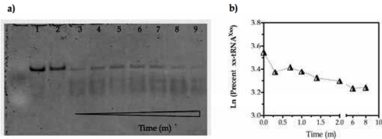
Fig. 20. Polyacrylamide gel analysis of the hydrolysis of ValtRNA Val-488 :EF-Tu ternary complex with RNase A/ T1 cocktail. Ternary complex composed of ValtRNA Val-488 (0.5 μM) and EF-Tu (5.0 μM), RNase A/ T1 cocktail (1 x 10 -4 Units A & 4.0 x 10 -3 Units T1). Lane 1 ValtRNA Val-488 (0.5 μM), lane 2 ValtRNA Val-488 :EF-Tu (0.5 μM and 5.0 μM), lanes 3 – 9 corresponds to reaction run times of 0.3, 0.7, 1, 1.4, 2, 6 and 8 minutes, respectively. Each reaction was quenched with unfractionated yeast total tRNA (1.0 mg/ mL). Gel conditions: 15% tris boric acid gel, 1X TBE running buffer (90 mM Trisma, 90 mM boric acid and 2 mM EDTA), run time 4 hours at 4°C.
