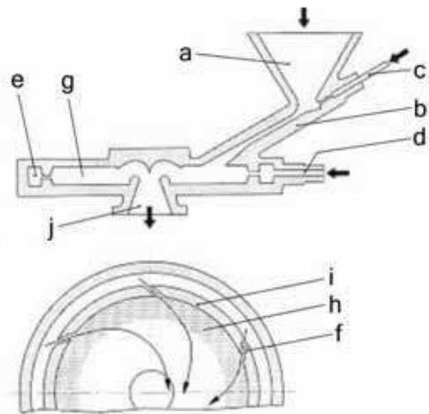
Fig. 2. Air jet mill 2 : funnel (a), injector (b), drive air (c), milling air (d), air ring (e), jet apertures (f), mill chamber (g), spiral air jets (h), jet ring wall (i), outlet (j)
