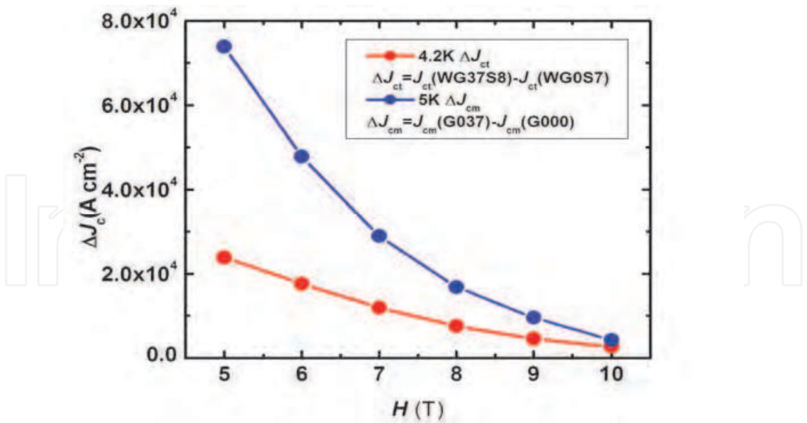
Fig. 6. Compared to the increment of magnetic J_{cm} at 5K and transport J_{ct} at 4.2K
