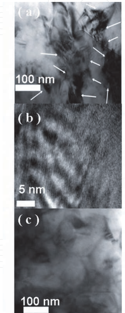
Fig. 11. (a) TEM image showing the defects with grains of the G037 sample with order of fringes varies between grains. Defects and fringes are indicated by arrow, and (b) HRTEM image of fringes. TEM images show large amount of defects and fringes can be observed in the graphene doped sample G037. (c) TEM image of the undoped sample for reference (Xu, X. et al., 2010).
