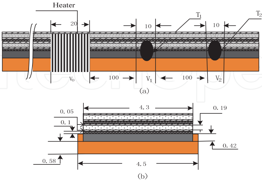
Fig. 16. Schematic of sample test arrangement. (a) and (b) are front-view and side-view of the hybrid conductor, respectively. T 1 and T 2 refer to temperature sensors. unit: mm.
