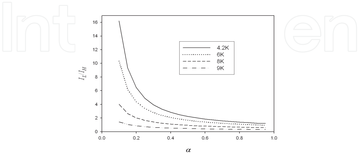
Fig. 7. The current ratio of NbTi to YBCO CC at different normalized transport currents
