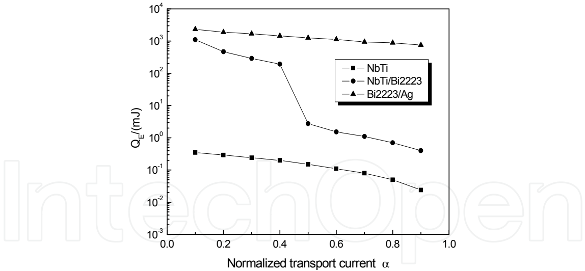
Fig. 14. MQE Q_E of three types of conductors
