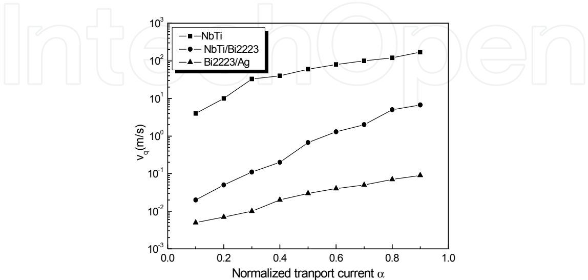
Fig. 13. Longitudinal QPV ( V_q ) of three types of conductors
