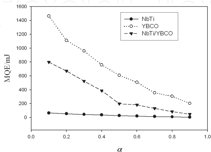
Fig. 11. The comparison of the MQE of NbTi, YBCO CC and NbTi/YBCO CC hybrid conductor with different transport currents.
