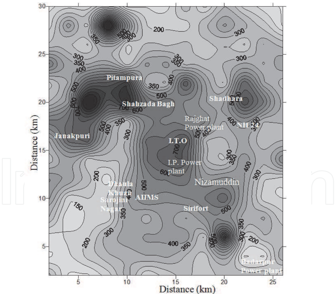
Fig. 6. 24 hourly averaged concentration of RSPM (µg/m³) due to all types of sources in Jan 2008.
