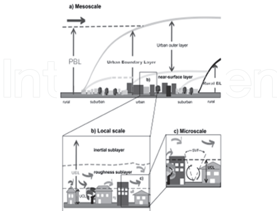
Fig. 2. Schematic diagram showing processes, flow and scale lengths within an urban boundary layer, UBL. This is set in the context of the planetary boundary layer, PBL, the urban canopy layer, UCL, and the sky view factor, SVF, a measure of the degree to which the sky is obscured by surrounding buildings at a given point which characterises the geometry of the urban canopy. Ref.: Meteorology applied to urban pollution problems-Final report COST Action 715. Dementra Ltd Publishers
