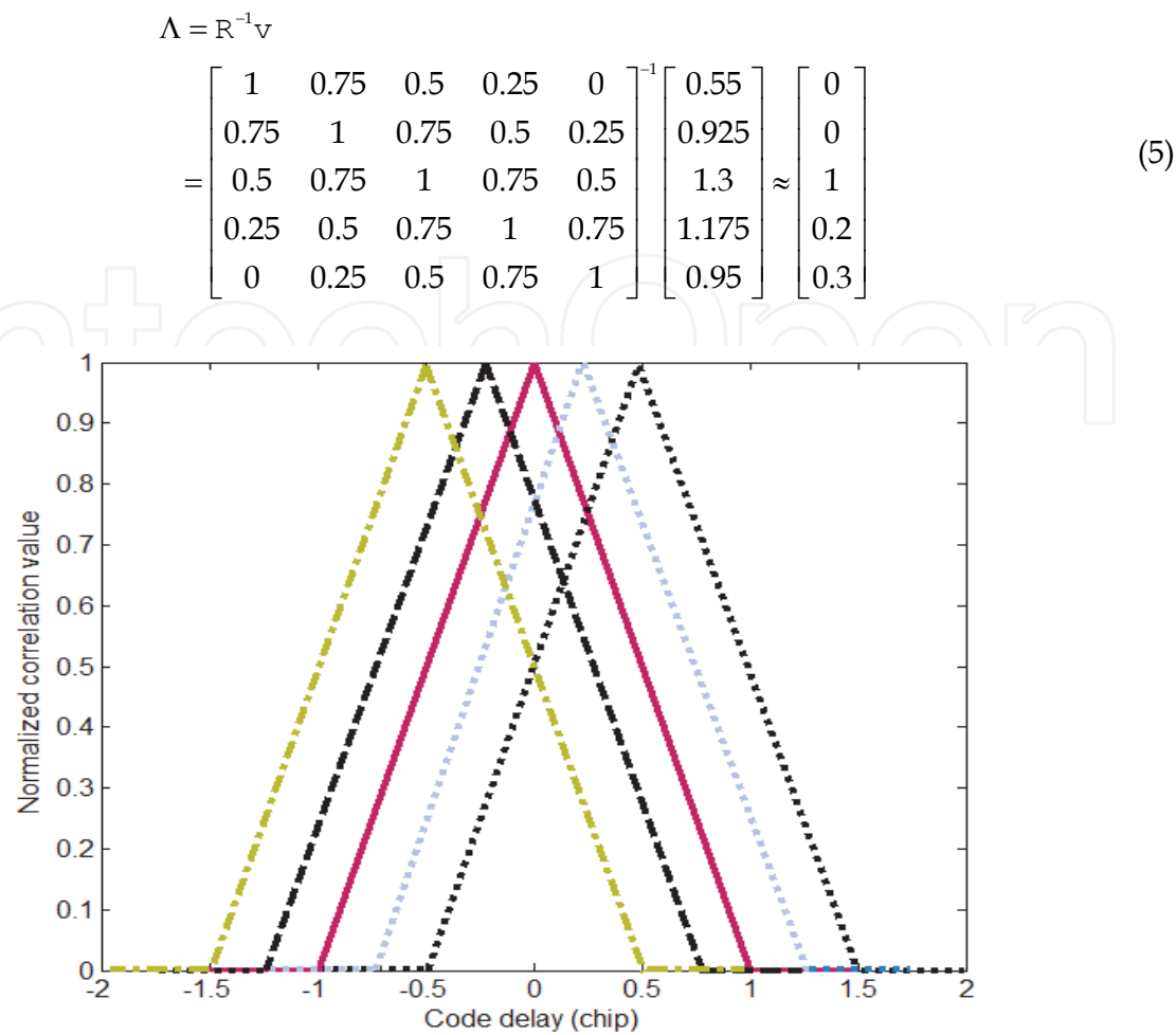
Fig. 4. Distribution of five correlators.
