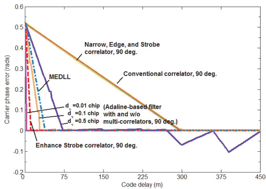
Fig. 12. Carrier phase error simulation results. ( \alpha_0 = 1.0, \alpha_1 = 0.5, \tau_0 = 0 chip, \tau_1 = 0 \sim 1.5 chip, \theta_0 = 0^\circ, (\theta_1 = 0^\circ, 180^\circ) ); delay element d_\tau = 0.01 chip, 0.1 chip, and 0.5 chip with and without multi-correlators.)
