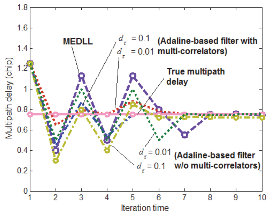
Fig. 13. Delay estimated by MEDLL and proposed method with and without multi-correlators. Note that Fig. 11 reveals that every DLL structure lacks of performance enhancement for short delay multipath signals. Nevertheless, the proposed method with multi-correlators can perform better in short delay and medium-to-long-delay multipath environment.
