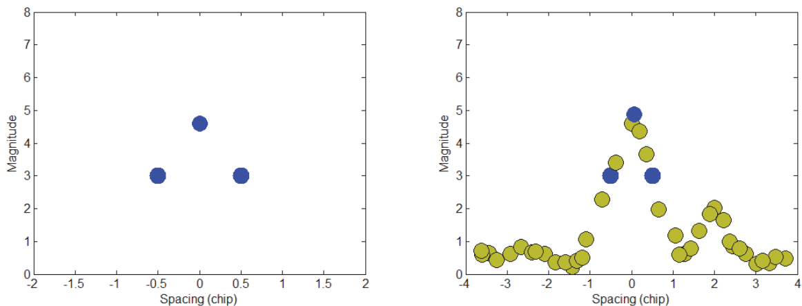
Fig. 3. Comparision of single correlator and multi-correlator.
