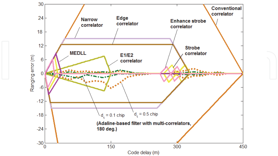
Fig. 11. Code-phase error simulation results of existing methods. ( \alpha_0 = 1.0 , \alpha_1 = 0.5 , \tau_0 = 0 chip, \tau_1 = 0 \sim 1.5 chip, \theta_0 = 0^\circ , (\theta_1 = 0^\circ, 180^\circ) ).
