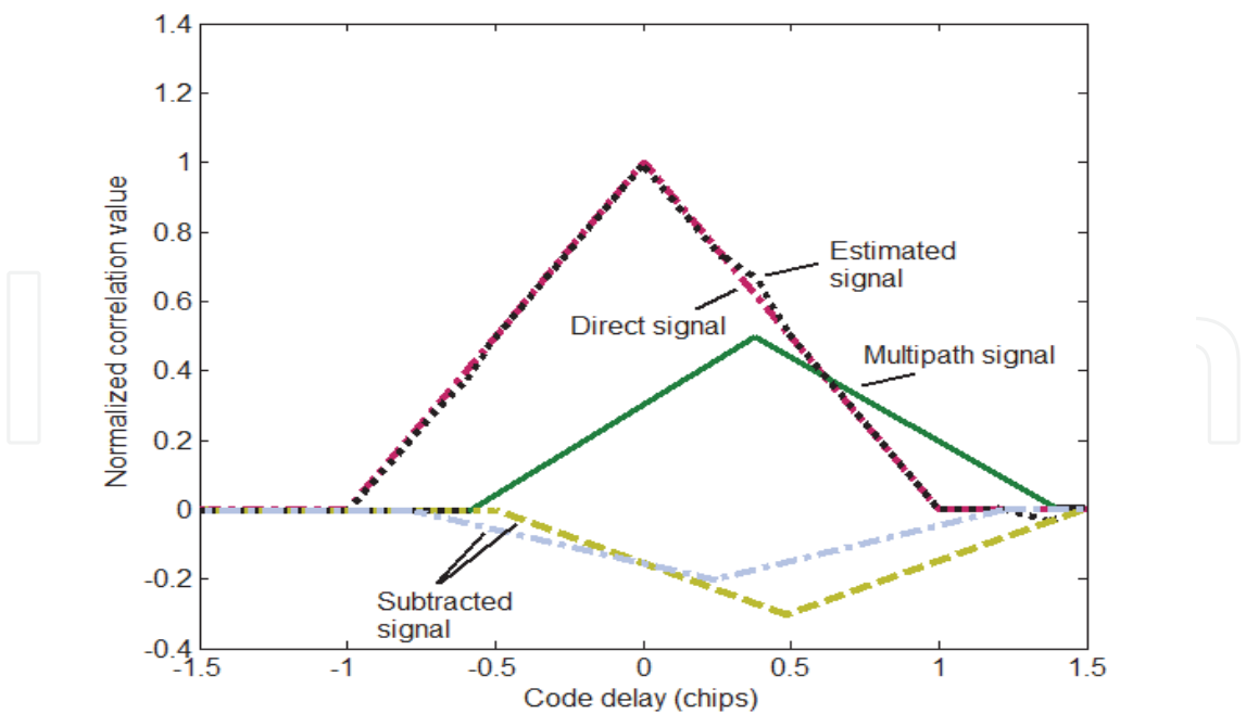
Fig. 6. Multipath delay is not at the set correlator.
