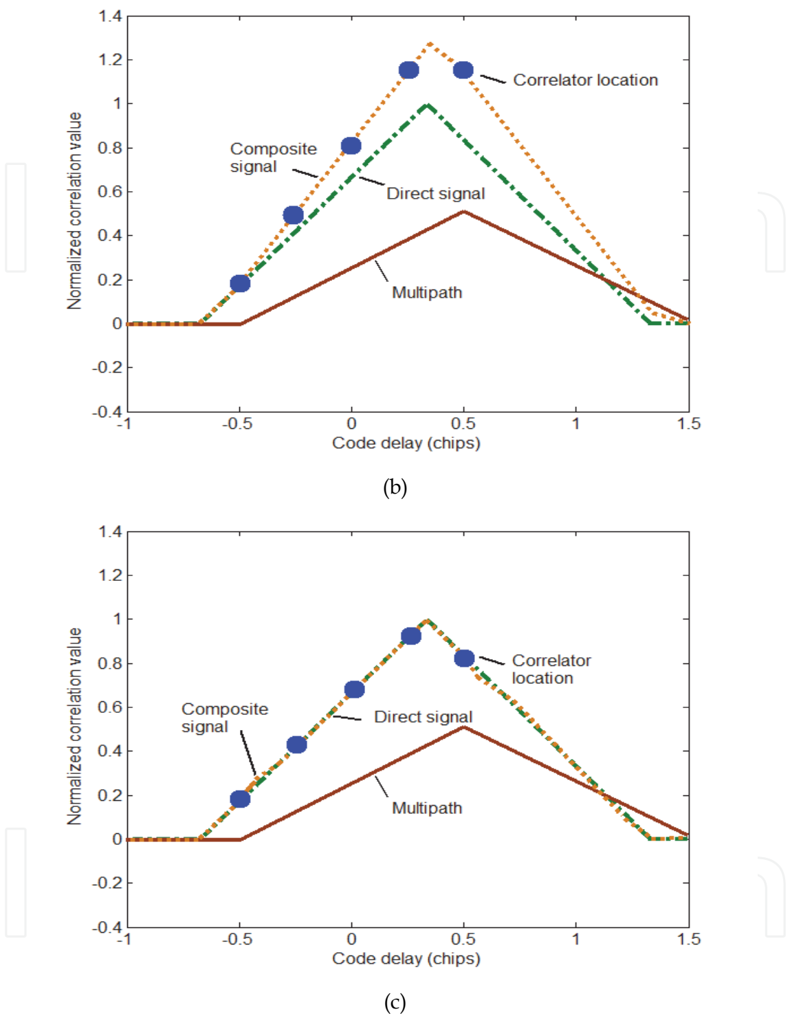
Fig. 8. Multi-correlators technique simulation results. (a) N=0, D=0.1 (b) N=1, D=0.1 (c) N=3, D=0.1 .
