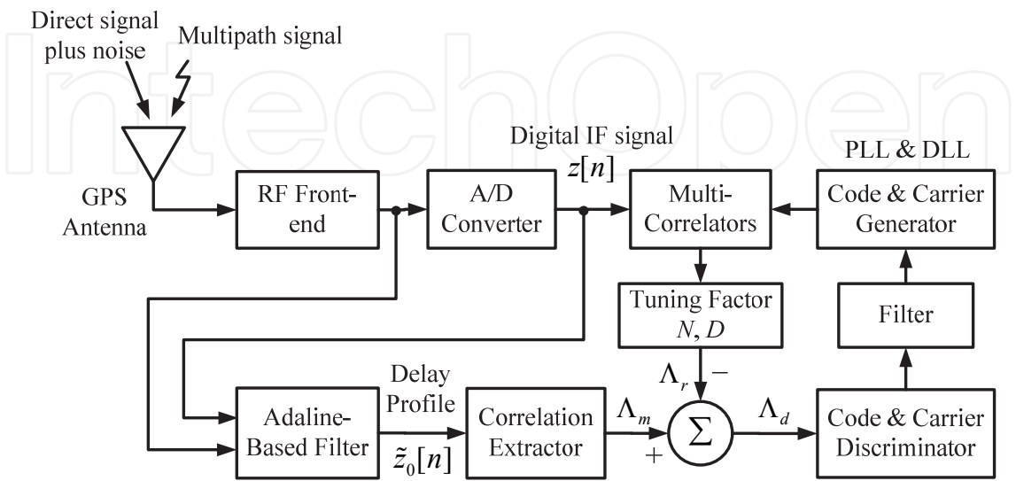
Fig. 7. Multipath Mitigation System Block Diagram.
