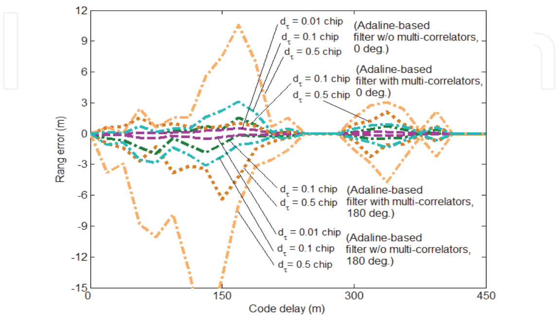
Fig. 10. Code-phase error simulation results of proposed method. ( \alpha_0 = 1.0 , \alpha_1 = 0.5 , \tau_0 = 0 chip, \tau_1 = 0 \sim 1.5 chip, \theta_0 = 0^\circ , (\theta_1 = 0^\circ, 180^\circ) ; delay element d_t = 0.01 chip, 0.1 chip, and 0.5 chip with and without multi-correlators.)
