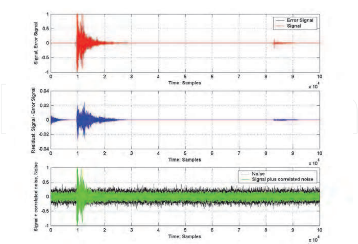
Fig. 10. Acoustic signal generated in high voltage chamber and received using Adaptive filter.
