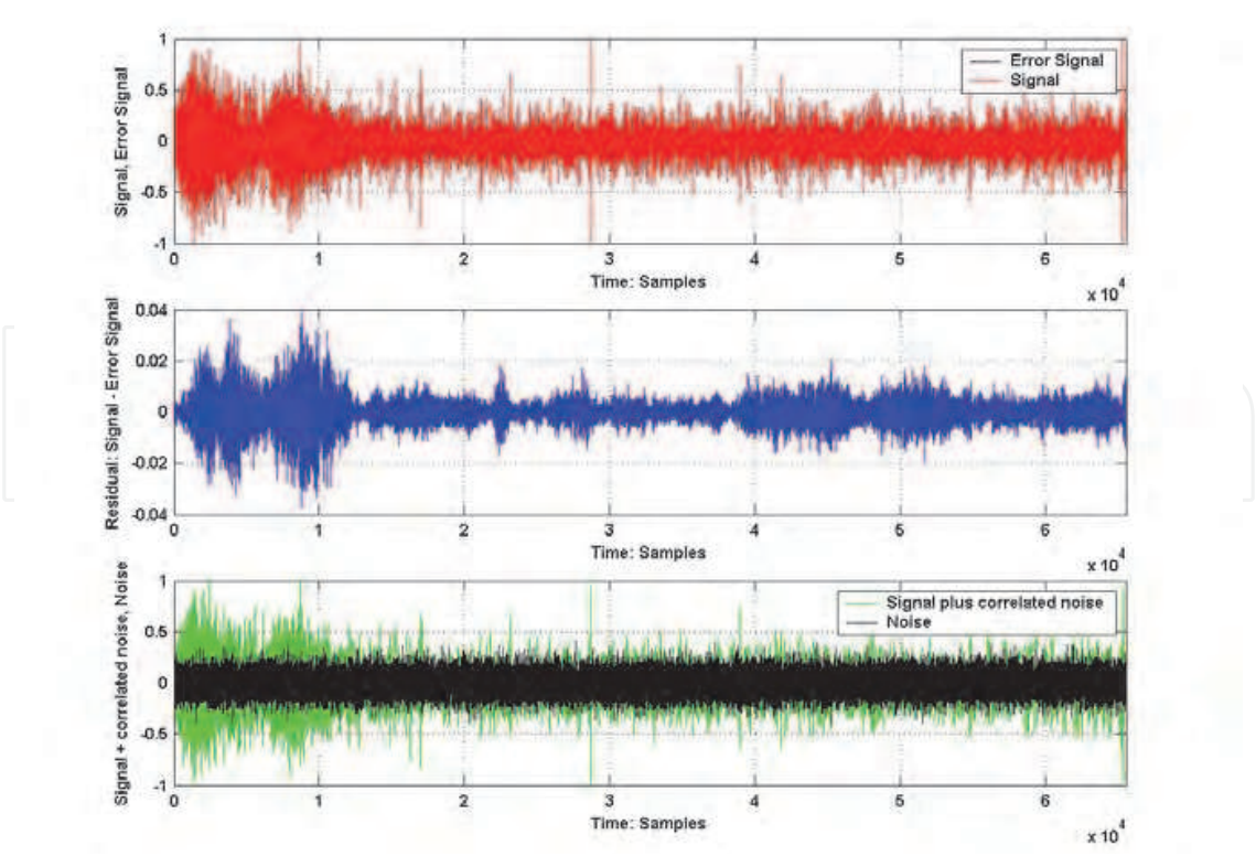
Fig. 11. TIPP event captured with Adaptive filter. The error signal is close to real input, an advantage of using AF to trigger on-board memory for saving noise-free transients.
