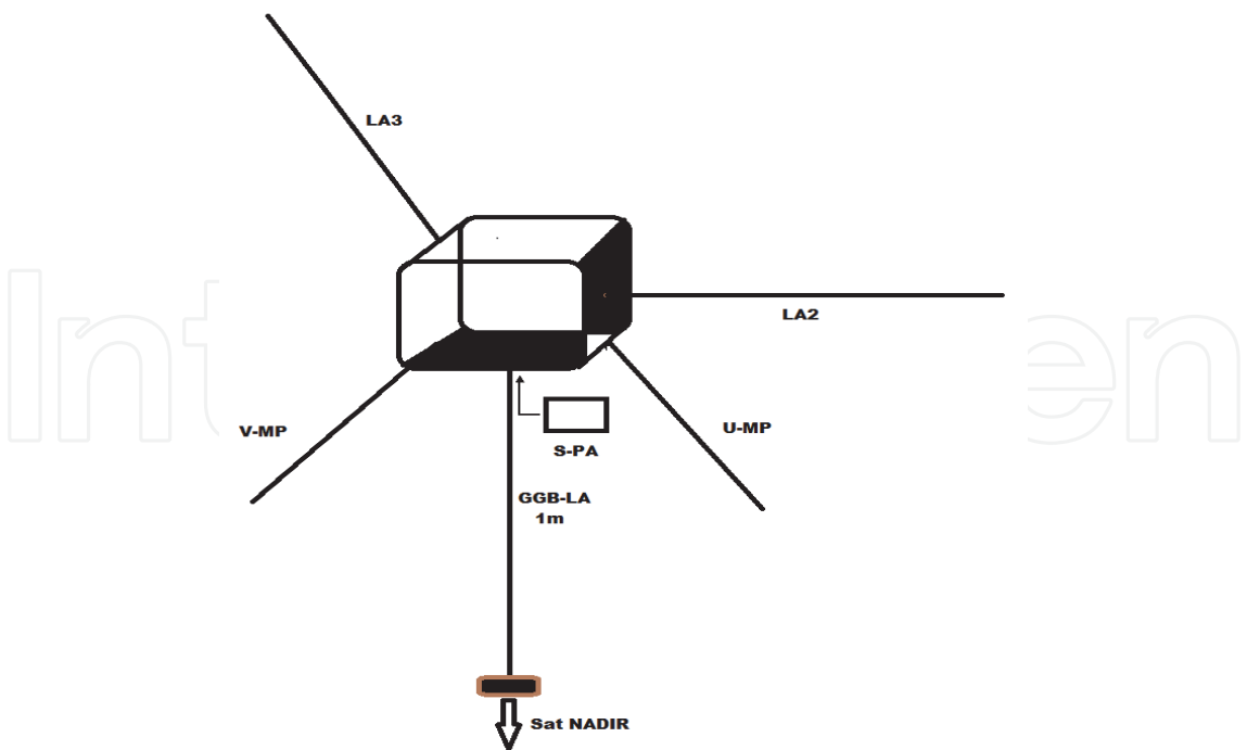
Fig. 5. LiNSAT structure with antenna configuration of three orthogonal lightning antennas (GGB-LA, LA2 and LA3). GGB is a passive attitude control sub-system to nadir direction. Additionally the multi-purpose boom is integrated as lightning antenna.
