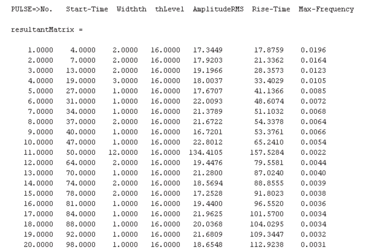
Fig. 12. Matlab™ simulated results of the program "lightning detector". In this computation, threshold level for coarse detection is set to 16 mV to extract all pulses above noise floor. Twenty pulses were detected along with their information about pulse start time, pulse rise/ fall time, amplitude and maximum frequency.
