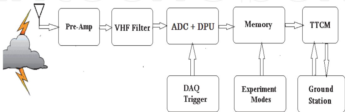
Fig. 8. Block diagram of LiNSAT scientific payload.
