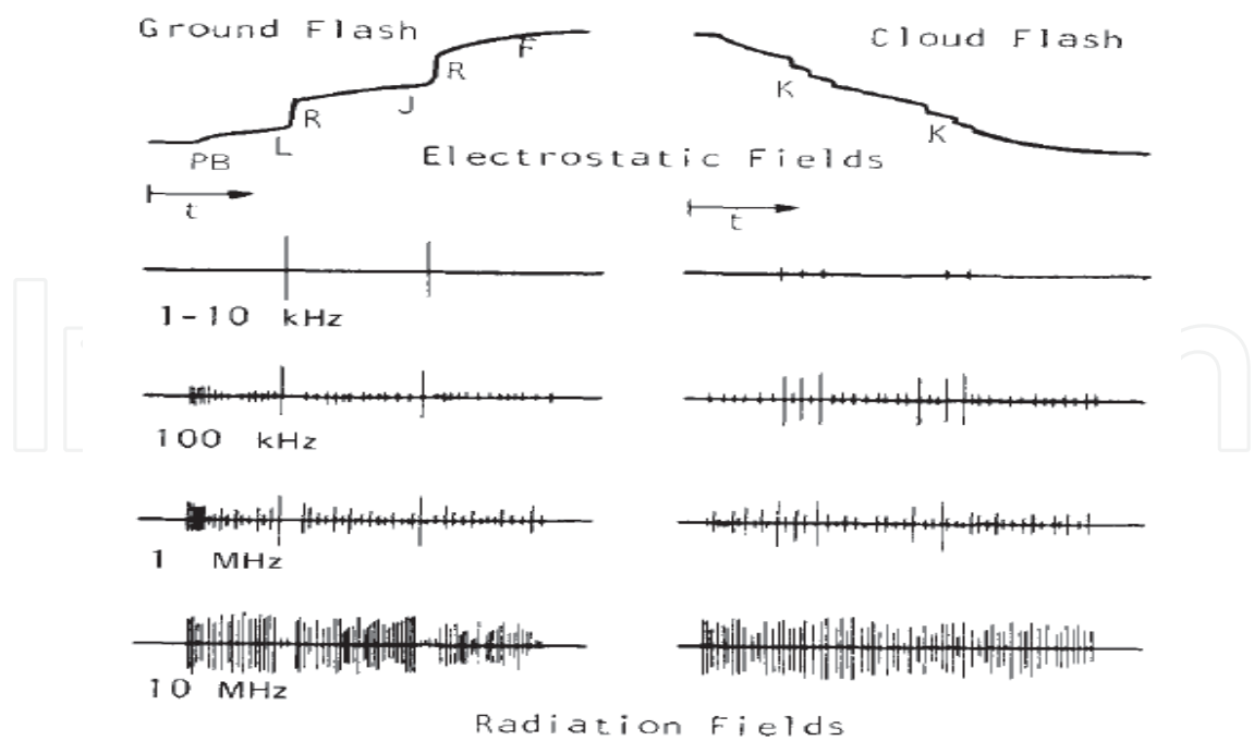
Fig. 4. Electromagnetic fields in lightning associated different channels, Preliminary Breakdown (PB), Leader (L), Return Stroke (R), Changes in (J, F and K). Adapted from ((Le Vine 1987)).
