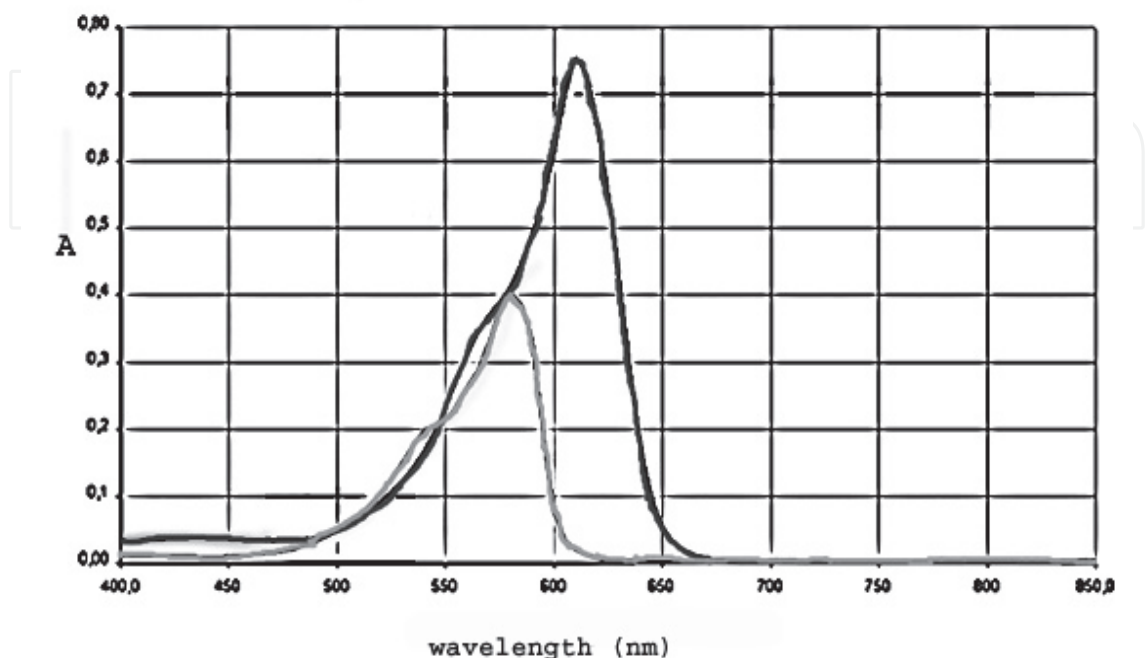
Fig. 6. Specific absorbance wavelengths of resazurin (—) and resorufin (---)
