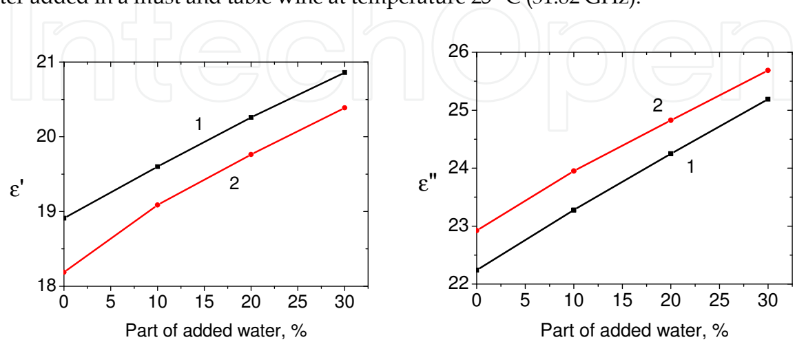
Fig. 9. The complex permittivity of the grape table wine (Rkatsitely) and must (from white Rkatsitely grape) with different degree of water dilution. The real (left) and the imaginary (right) complex permittivity parts. The numbers denote: 1 – must, 2 – wine.
