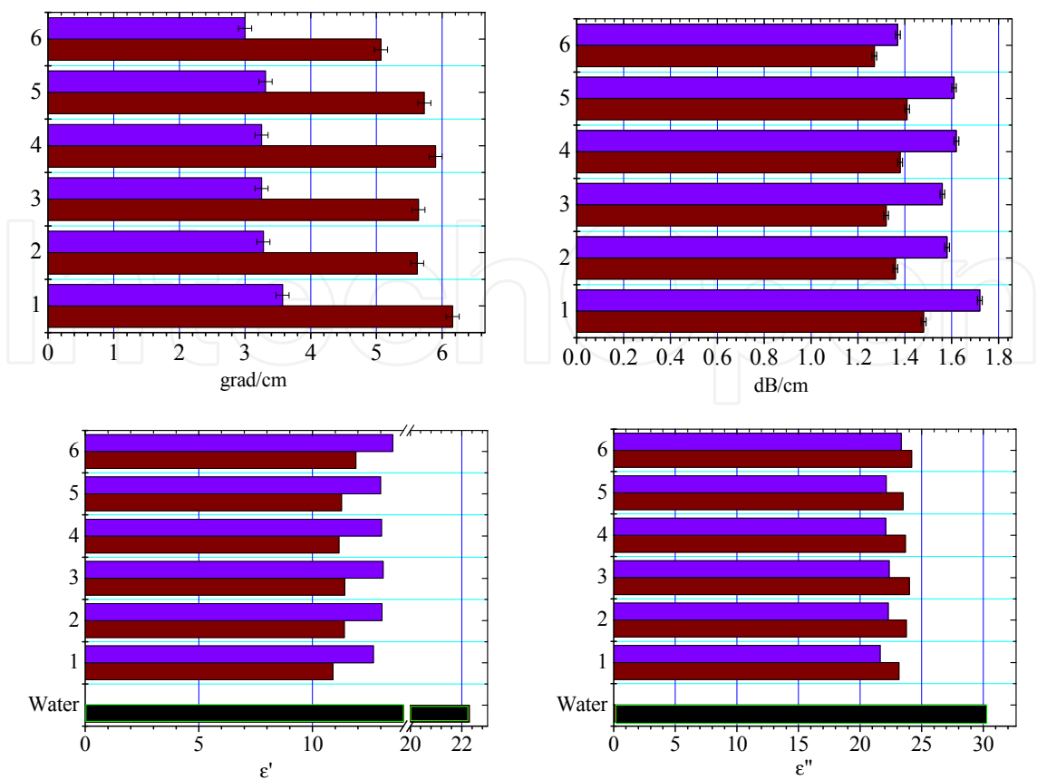
Fig. 5. The increment of the wave phase (upper left) and the attenuation (upper right) coefficients in the cell with water and in the cell with table wines (musts) with respect to the distilled water are presented. There are the real (bottom left) and imaginary (bottom right) complex permittivity parts of wines and musts samples, respectively. In blue there are data for musts, in brown there are data for wines. The data of grapes vintage are shown on the vertical axis such as 1 - Chardonnay 8 Sept. 07, 2 - Aligote 14 Sept. 07, 3 - Riesling Rhine 12 Sept. 07, 4 - Riesling Rhine 19 Sept. 07, 5 - Riesling Rhine 20 Sept. 07, 6 - Rkatsiteli 27 Sept. 07.
