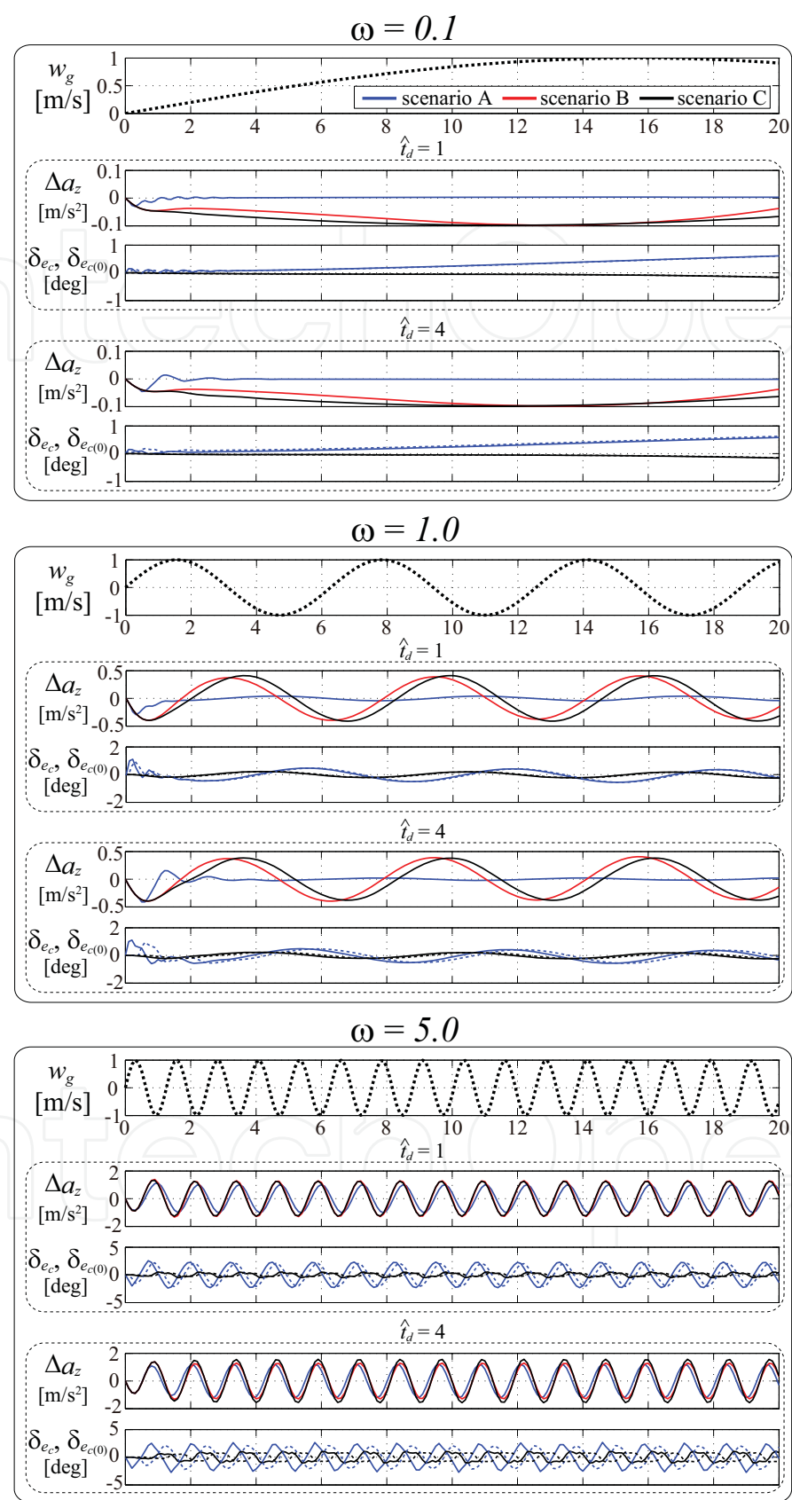
Fig. 4. Time histories under no measurement errors in turbulence data with R = 10^2 and N = 20 ( \delta_e is shown as dotted lines and \delta_{e(0)} is shown as solid lines)
