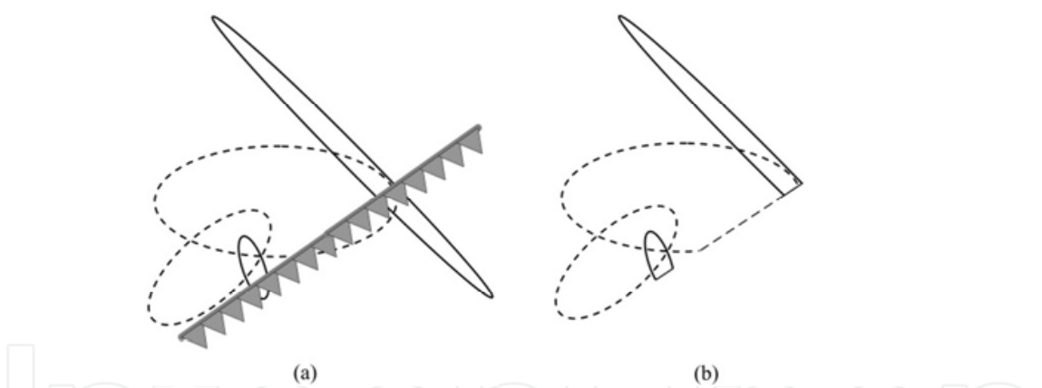
Fig. 4. Uncertainty error ellipses are affected by sensor blockage. a) Gaussian ellipses and blockage indicated; b) resulting alteration of ellipse.
