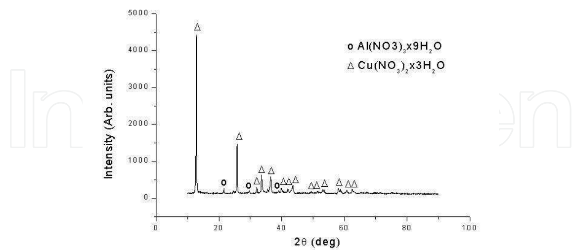
Fig. 3. XRD of the Cu-3wt.%Al 2 O 3 powder after spray-drying
