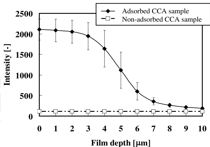
Fig. 9. Relationship between the depth of CCA sample and fluorescent intensity derived from perylene/GTA mixture obtained under conditions of high-speed-mode, \pm 10\ \mu\text{m} range and 1\ \mu\text{m} intervals.
