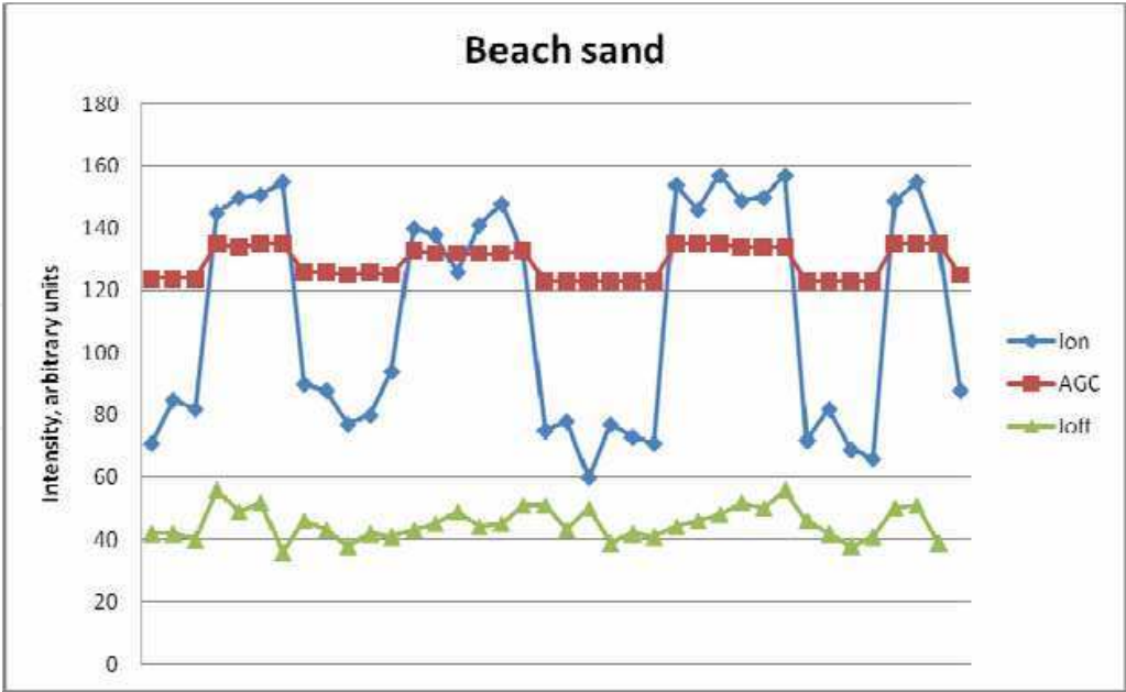
Fig. 9. AGC effect on intensity. Beach sand data collected from Hyytiälä, Finland. Blue line represent the intensity values when the AGC was turned on, red line is the AGC values itself and the green line is the intensity values when the AGC was turned off. (Vain et al., 2010)
