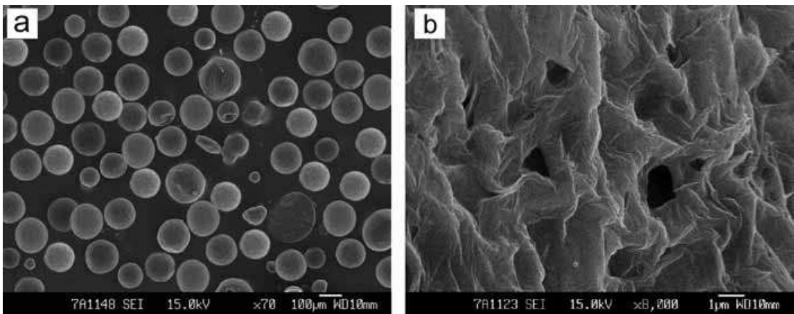
Fig. 5. Scanning electron micrographs of PHBBMA .(a) whole particles (×70) and (b) surface of particle (×8000). ( Zhang et al., 2010b)
