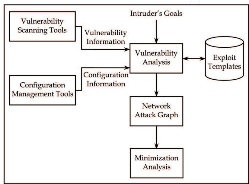
Fig. 1. Minimization analysis of network attack graphs
