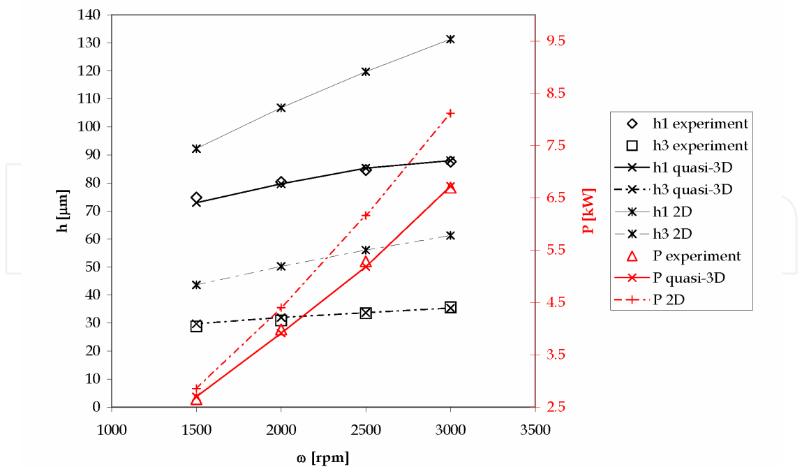
Fig. 10. Power loss ( P ) and film thickness at pad inlet ( h_1 ) and outlet ( h_3 )
