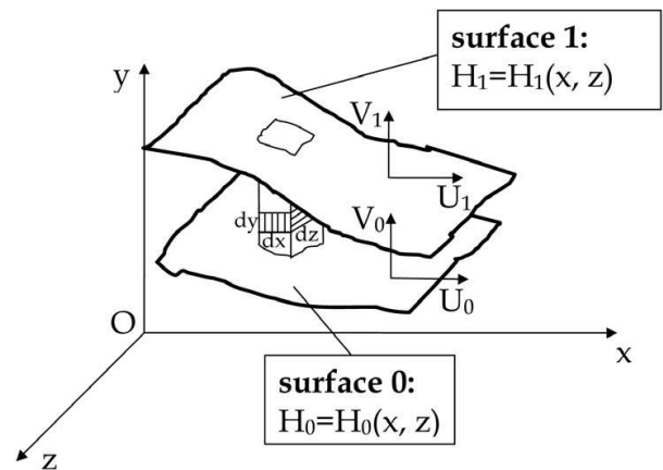
Fig. 1. Reference system O(x, y, z) and flow between the two surfaces 0 and 1 moving with velocity \mathbf{V}_0=\{U_0, V_0, 0\} and \mathbf{V}_1=\{U_1, V_1, 0\}
