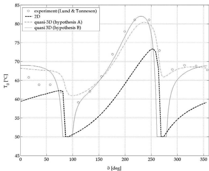
Fig. 7. Centerline temperatures on the bearing surface calculated by means of the 2D model and the quasi-3D model (two-axial groove journal bearing, \omega=5000 rpm, F_X=5600 N) external temperature ( T_s=50^{\circ}\text{C} , T_e=20^{\circ}\text{C} ) and, therefore, the thermal simulation requires the calculation of the term T_0 in eq. (52) in order to fulfil hypothesis B. Accordingly T_0=T_e has been imposed on \Omega_g while calculating the corresponding sensitivity matrix (term S_0 in eq. (52)). The adoption of either hypothesis A or B enables the heat exchange between the structure of the bush and the lubricant in the grooves to be simulated. The lack of such modelling detail causes, in the present case, a bush peak temperature overestimation of roughly 10^{\circ}\text{C} . Although hypothesis A yields a better temperature trend than hypothesis B, it leads to an underestimation of the journal temperature that is evident in the cited Lund’s paper too. A comparison among journal temperature results is reported in Table 1, where axially averaged values are calculated for the one-dimensional journal sub-models adopted in the quasi-3d analyses (see the reference paper for details).
