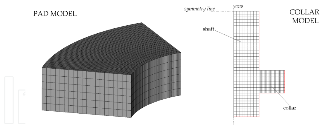
Fig. 8. Finite element models of the thrust pads and the shaft-collar assembly
