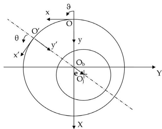
Fig. 2. Cylindrical pair (complete journal bearing) with ideal (rigid) members and reference systems
