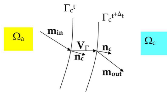
Fig. 5. Mass flows through the moving cavitation boundary
