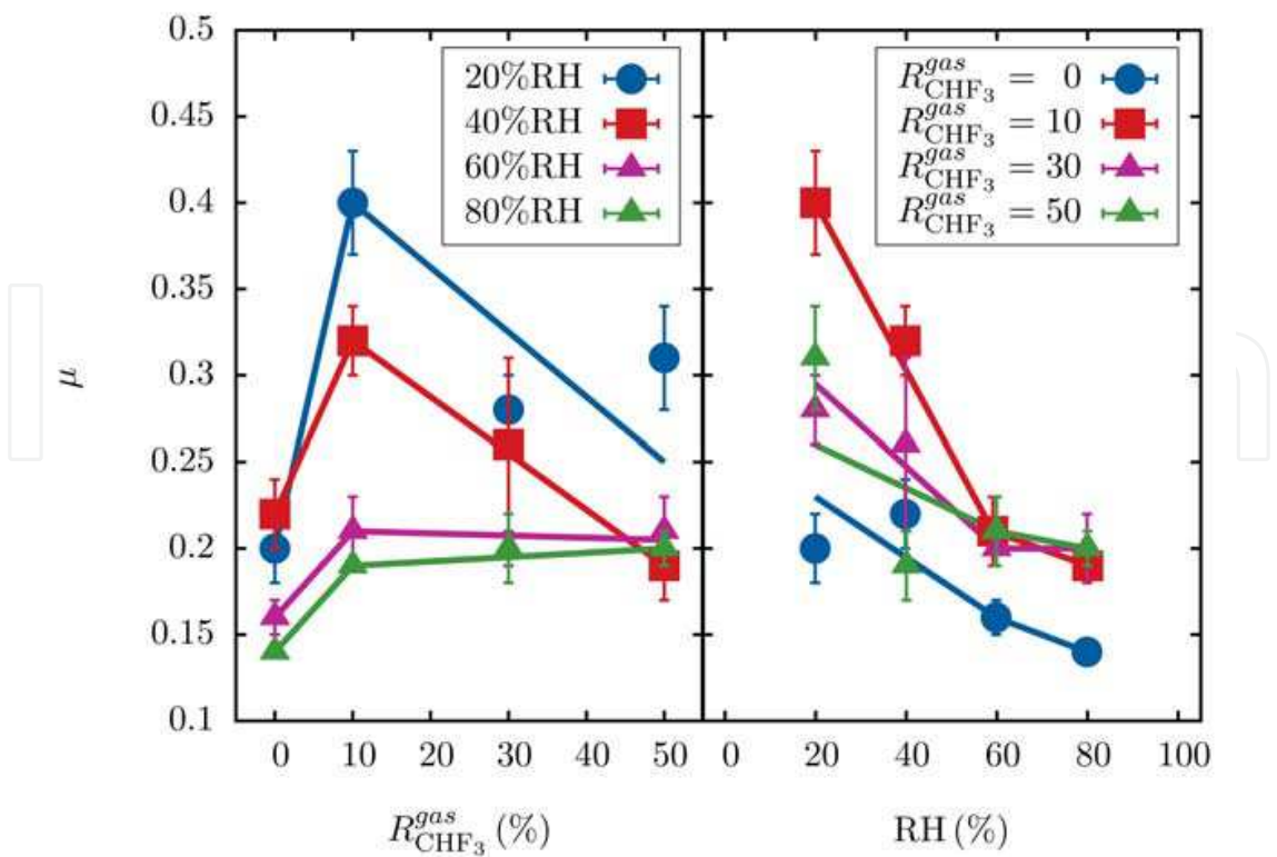
Fig. 6. Friction dependence on humidity and fluorination degree.
