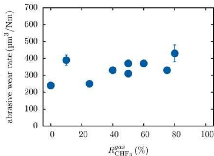
Fig. 7. Abrasive wear rate of the films after 6 min with a 1:3 suspension of alumina particles 1\ \mu\text{m} in diameter in glycerin, with a load of 0.54\ \text{N}
