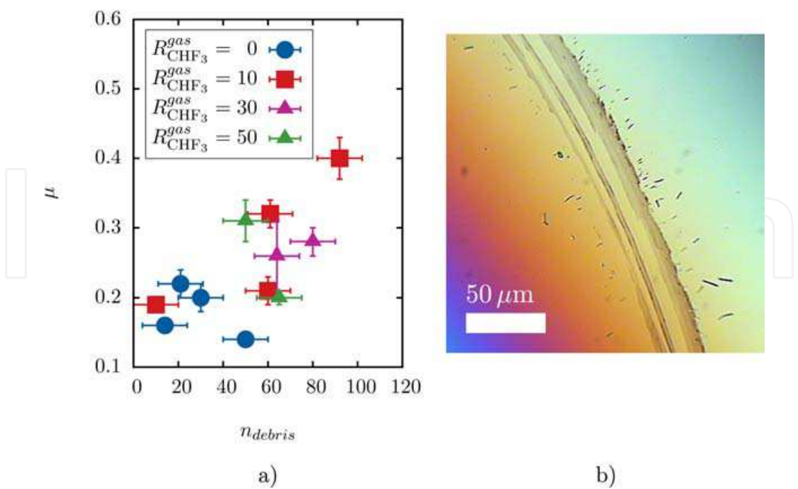
Fig. 5. a) Friction vs number of debris particles visible at 50× (200×200 \mu m ).The dependence of friction with number of particles is only clear for high friction values; b) 50× optical microscope picture of a typical sliding track, corresponding to a film with R_{CHF_3}^{gas} = 10\% measured CHF_3 at 60% RH. Fiber-like debris particles are present at both sides of the sliding track.
