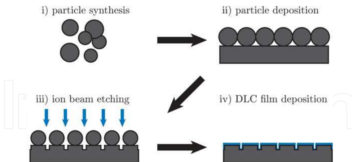
Fig. 8. Fabrication process of DLC films with patterned surface: i) Synthesis of silica particles; ii) Particle deposition by Langmuir-Blodgett (colloidal template); iii) Pattern transfer to the substrate surface ( \text{Ar}^+ beam etching); iv) DLC film deposition on the patterned substrate.
