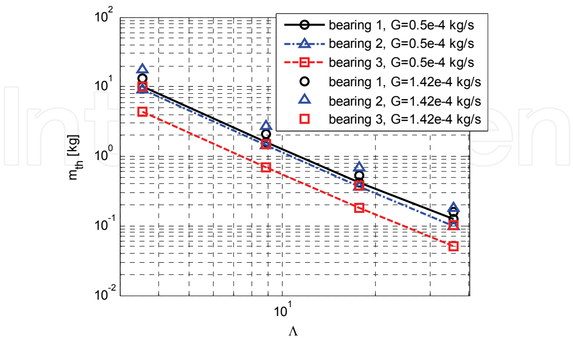
Fig. 17. Rotor mass m at stability threshold vs. bearing number \Lambda for the three bearings
