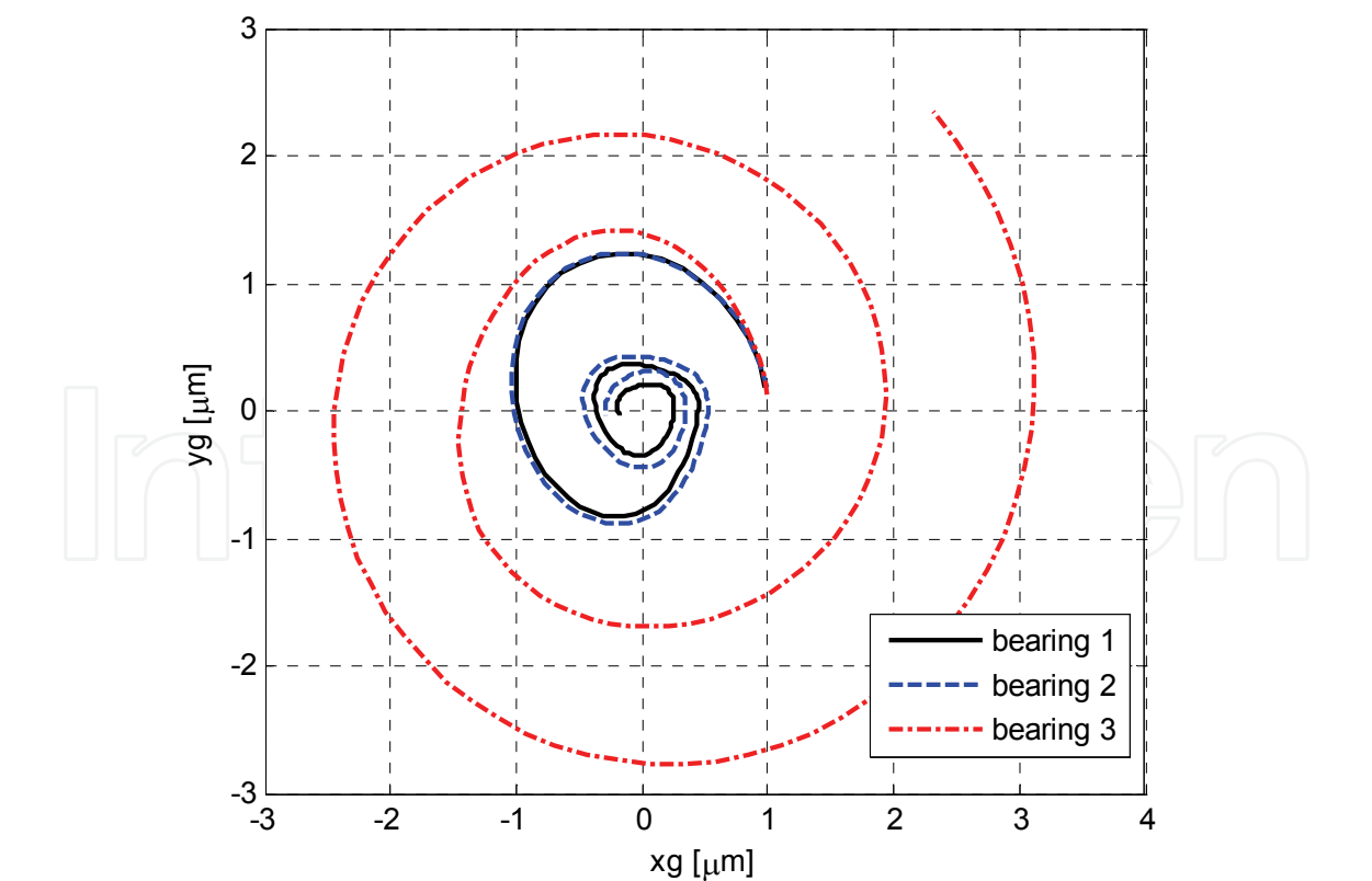
Fig. 12. Rotor trajectories with the three bearing types; m=1 kg, \omega=50 krpm; initial conditions x(0)=1\text{ }\mu\text{m} and dy/dt(0)=x(0)\cdot(k_{xx}/m)^{(0.5)} .
