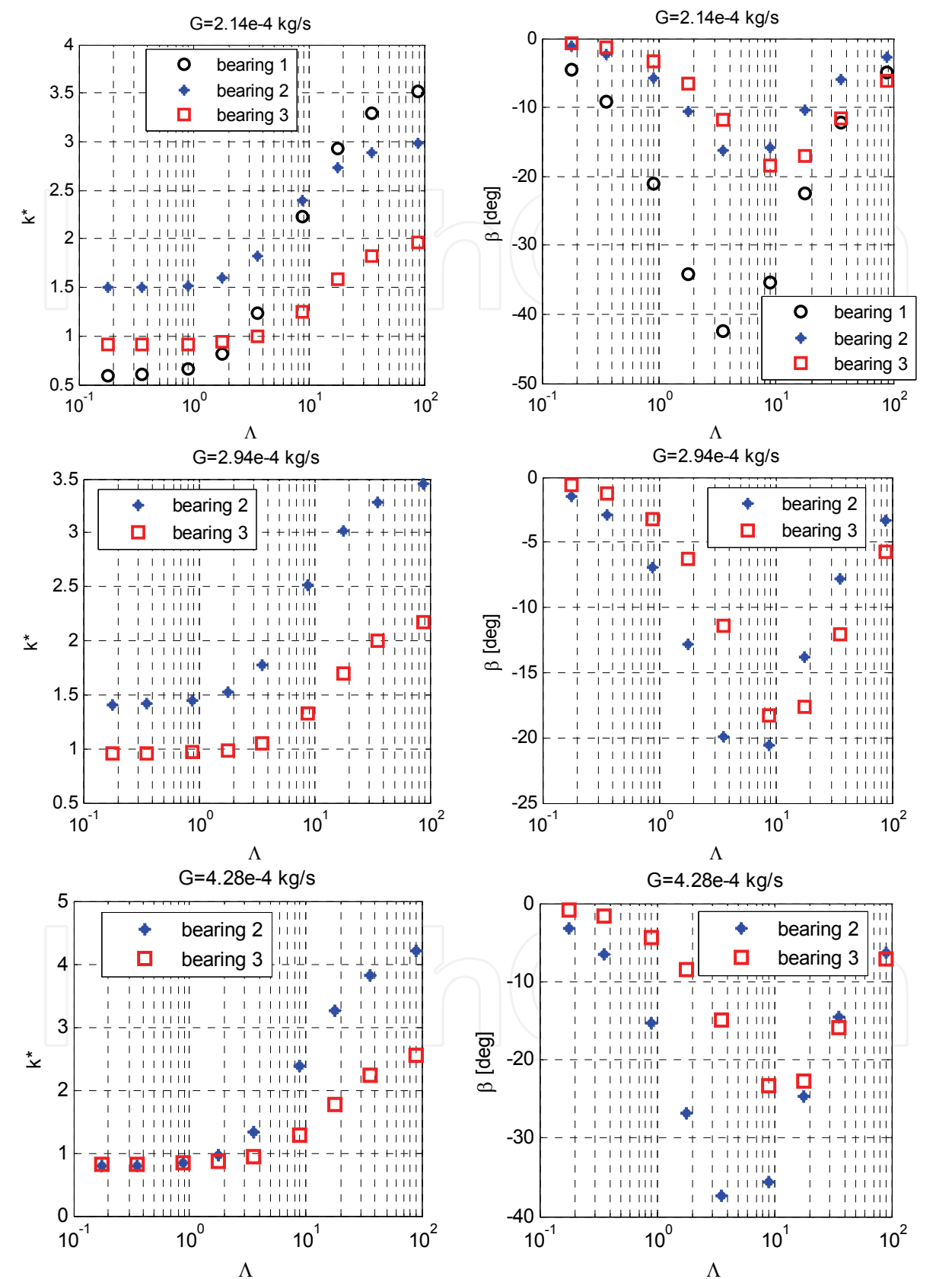
Fig. 9. Non-dimensional bearing stiffness k^* and attitude angle \beta vs. bearing number \Lambda for the three bearings
