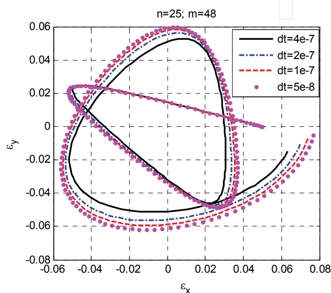
Fig. 3. Rotor trajectories with bearing type 1 obtained with different time steps and grid 25x48; initial conditions specified by \varepsilon_x(0)=0.05 , \varepsilon_y(0)=0 , \dot{\varepsilon}_x(0)=0 , \dot{\varepsilon}_y(0)=0 , h_0=20 \mu\text{m} , p_s=5 \cdot 10^5 Pa rel., d_s=0.1 mm, \omega=60 krpm
