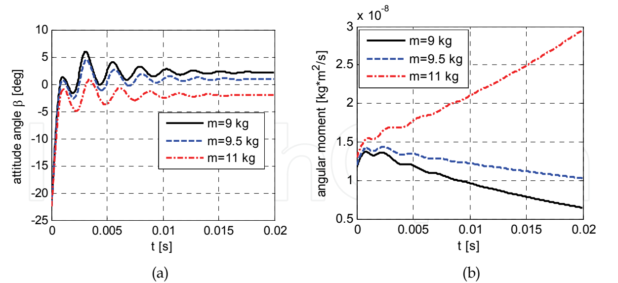
Fig. 11. Attitude angle vs. time (a) and rotor angular moment vs. time (b) with different rotor masses and initial condition x(0)=1\text{ }\mu\text{m} , dy/dt(0)=x(0)\cdot(k_{xx}/m)^{(0.5)} ; \omega=20 krpm, bearing type 1 The three bearings are compared in figures 12 and 13, showing the rotor trajectories for identical initial condition, the attitude angle vs. time and the rotor angular moment vs. time. In this case bearing types 1 and 2 are very similar, while bearing type 3 is unstable.
