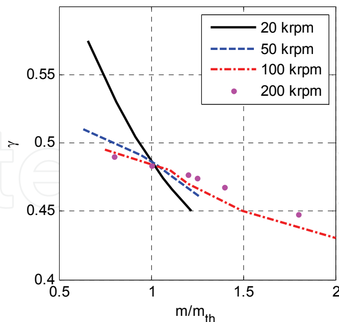
Fig. 16. Whirl ratio \gamma vs. m/m_{th} at different speeds; bearing type 1, G=0.5 \cdot 10^4 kg/s
