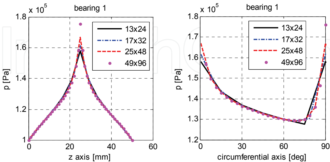
Fig. 2. Axial and circumferential pressure distributions for bearing type 1 obtained with different mesh grids; h_0=20 \text{ }\mu\text{m} , p_s=5 \cdot 10^5 \text{ Pa rel.} , d_s=0.1 \text{ mm} , \omega=60 \text{ krpm} , \varepsilon=0
