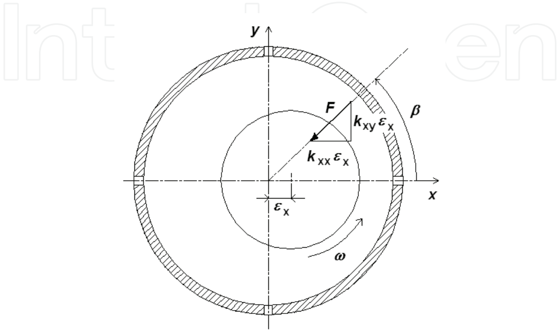
Fig. 8. Bearing reaction force on the journal in steady-state conditions due to shaft displacement along direction x
