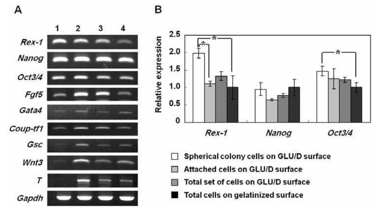
Fig. 4. RT-PCR analysis of ES cells cultured on different surfaces after four passages. (A) Conventional RT-PCR analysis for three markers of undifferentiated stem cells ( Rex-1 , Nanog , and Oct3/4 ) and six markers of early differentiation ( Fgf5 , Gata4 , Coup-tf1 , Gsc , Wnt3 , and T ). Lanes 1, 2, 3, and 4 correspond to the spherical colony cells, attached cells, and total cells cultured on the GLU/D surface, and the total cells collected from the gelatinized surface, respectively. (B) Quantitative RT-PCR analyses for the three stem cell markers ( Rex-1 , Nanog , and Oct3/4 ) in ES cells cultured on the GLU/D or gelatinized surface. The data were obtained from three independent experiments. The vertical bars show the standard deviation (* p < 0.05 )
