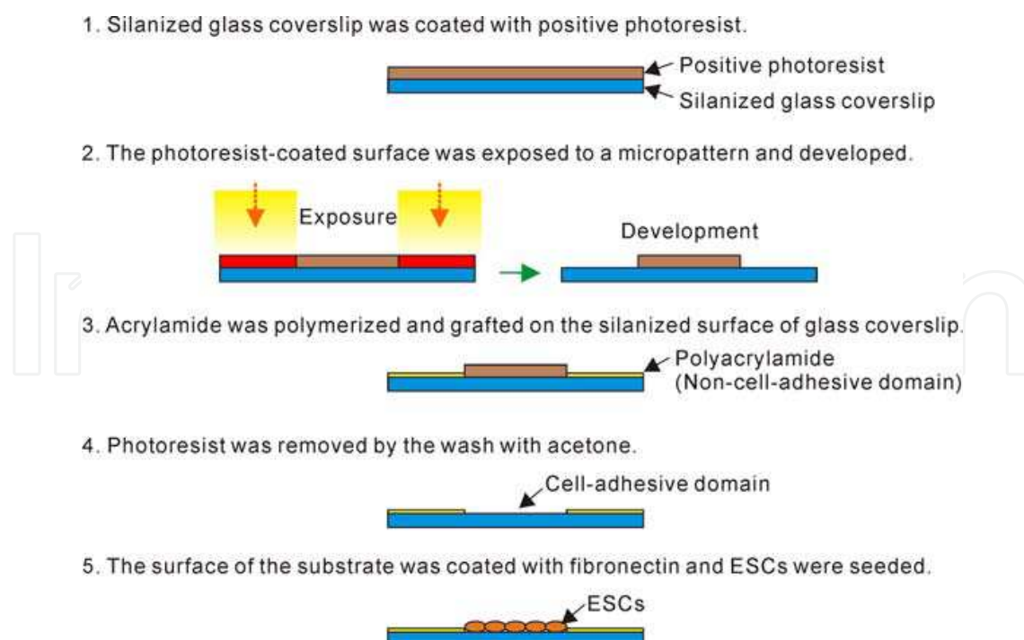
Fig. 2. Schema of the fabrication process of cell-patterning substrates.
