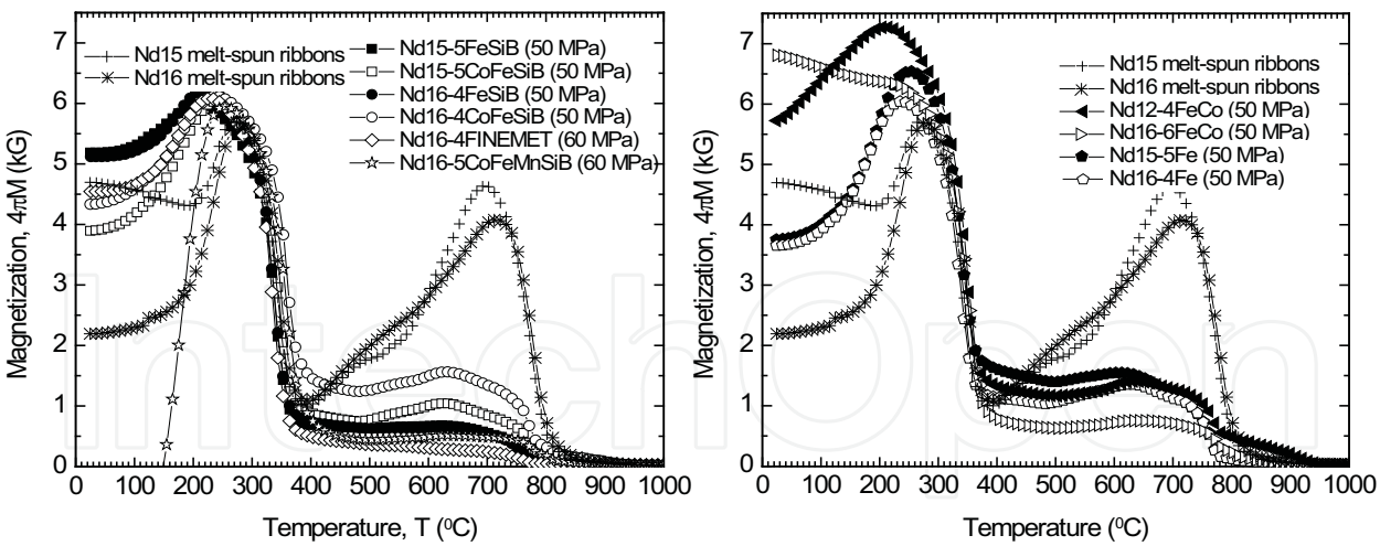
Fig. 9. M-T curves for Nd-Fe-B/soft magnetic powders SPS nanocomposite magnets. The thermomagnetic curves for Nd15 and Nd16 melt-spun ribbons are shown for comparison. The values of the magnetic characteristics for several Nd-Fe-B/FeSiB and Nd-Fe-B/CoFeSiB nanocomposite magnets prepared by SPS are shown in Table 3.
