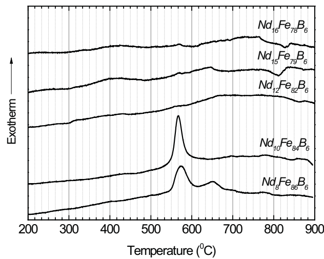
Fig. 2. DSC curves for Nd-Fe-B melt-spun ribbons vs. Nd content.
