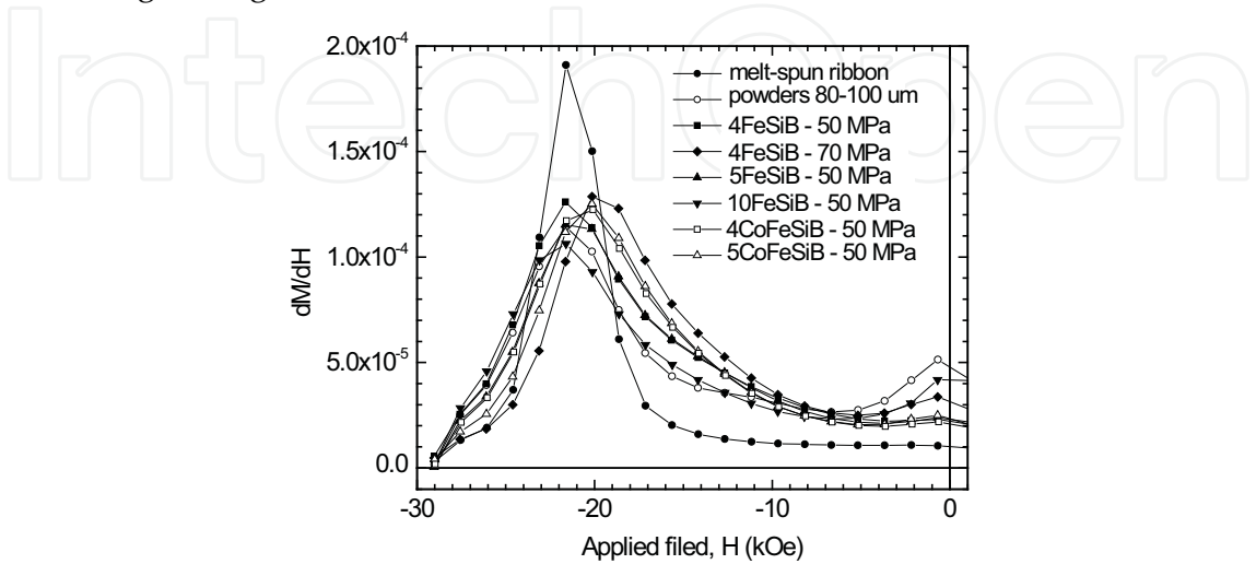
Fig. 11. dM/dH=f(H) curves for Nd16 melt-spun ribbons, ball-milled powders and SPS consolidated nanocomposite magnets as a function of added soft magnetic material (Lupu et al., 2009).
