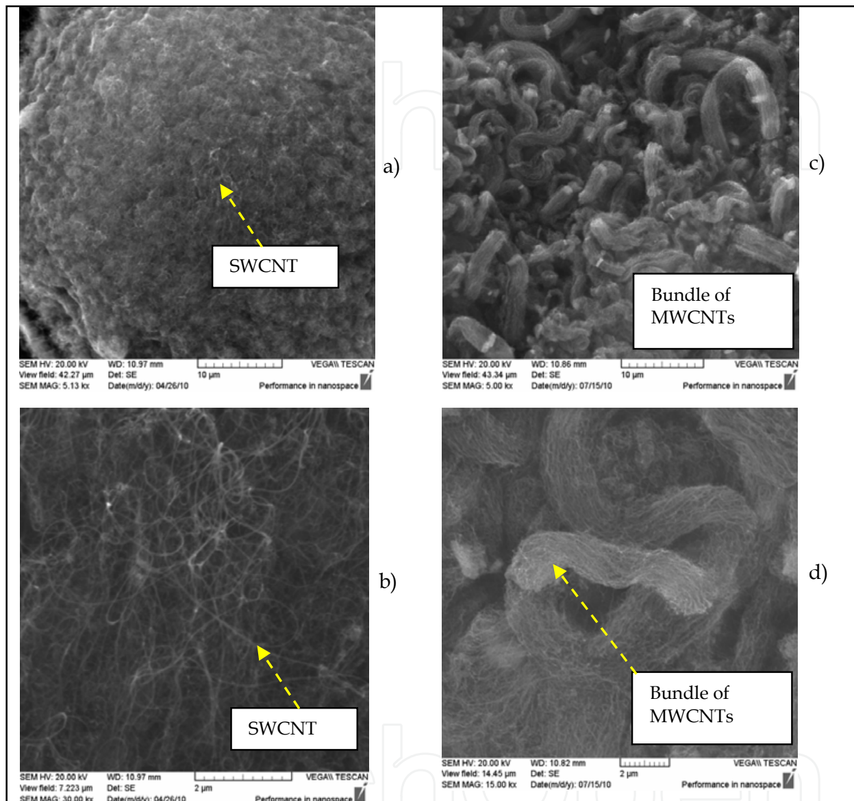
Fig. 2.1.1 a) SWCNTs zoom 5x (10µm scale), b) SWCNTs zoom 30x (2µm scale), c) MWCNTs zoom 5x (10µm scale), d) MWCNTs zoom 15x (2µm scale),
