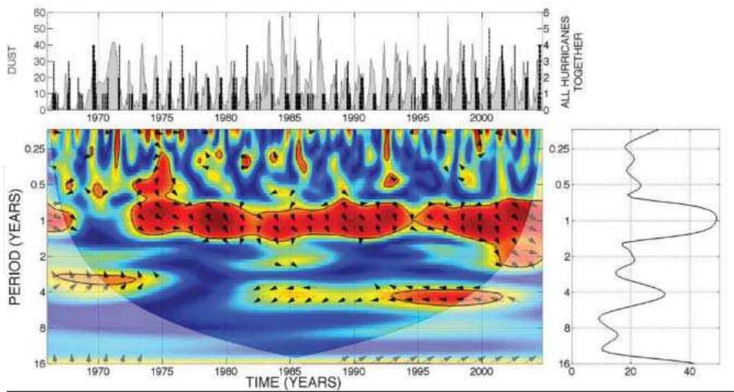
Fig. 13. Time series of African Dust (shaded area) - all hurricanes categories together (black bars). The lower panel is wavelet-squared transform coherency (WTC), and the right panel is the Global spectrum GXWT.
