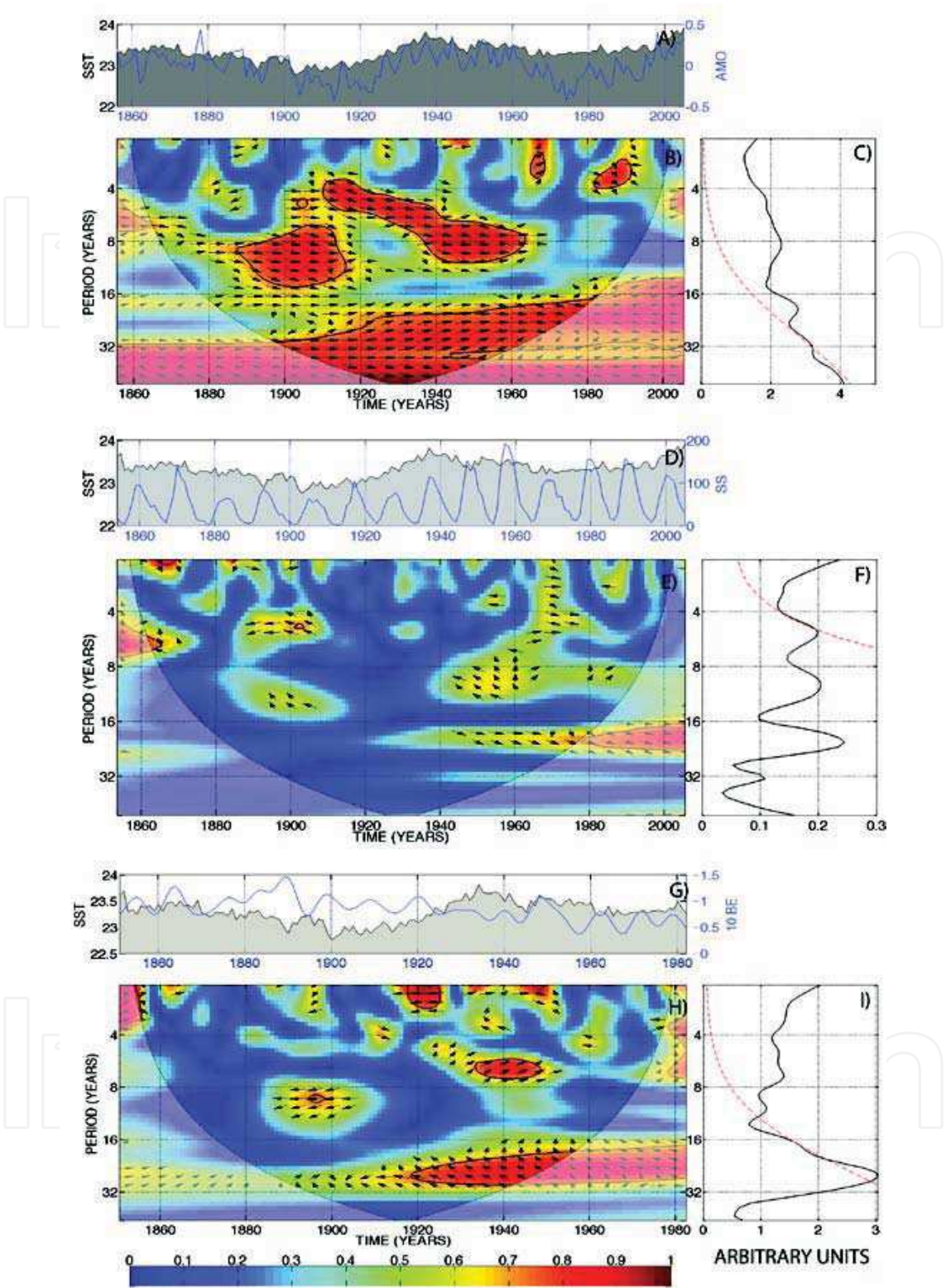
Fig. 8. (A) Time series of AMO (blue line) and SST (gray area). (B) Coherence between SST and AMO. (C) Significance level of the global spectra of SST and AMO. (D) Time series (blue line) of SS and SST. (E) Coherence between SST and SS. (F) Significance level of the global spectra of SST and SS. (G) Time series of SST and CR ( ^{10}\text{Be} ) (blue line). (H) Coherence between SST and CR ( ^{10}\text{Be} ). (I) Significance level of the global spectra of SST and CR ( ^{10}\text{Be} )
