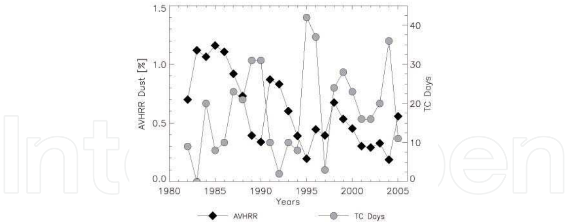
Fig. 6. Time series of North Atlantic tropical cyclone days and Saharan-induced dust cover for 1982-2005. The black line and diamonds represents the detected dust cover and the gray line and circles represents the tropical cyclone days, over the region of 030N and 1560W for the time period of August 20 through September 30 ((20)).
