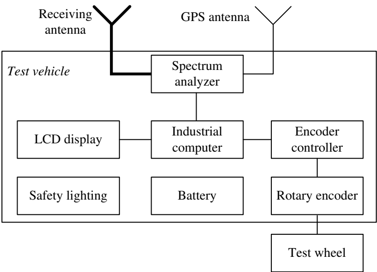
Fig. 7. Simplified block diagram of the mobile receiving section (Ambroziak, 2010)
