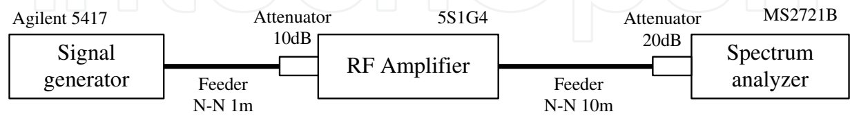
Fig. 3. Transmitting section calibration set schematic diagram
