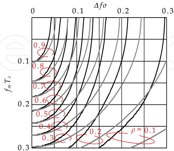
(c) Locus of theory (fine) & simulation(solid)
