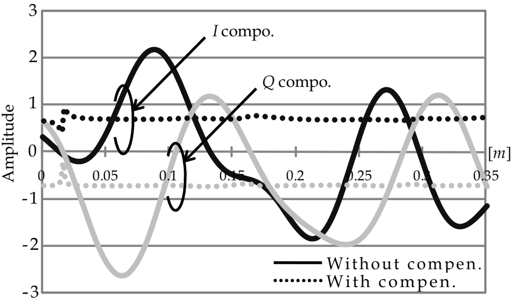
(a) I and Q components
