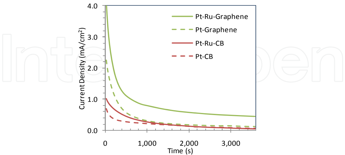
Fig. 5. Chronoamperogram curves for graphene- and carbon black-supported Pt and Pt-Ru nanoparticles in 1 M CH 3 OH/0.5 M H 2 SO 4 . The potential was 0.4 V vs. Ag/AgCl.
