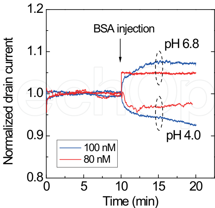
Fig. 11. Time course of normalized I_D for G-FETs at V_D and V_{TGS} of 0.1 and -0.1 V, respectively, in 10-mM phthalate and phosphate buffer solution. Red (blue) lines indicate that 80 (100) nM BSA was added at 10 min.
