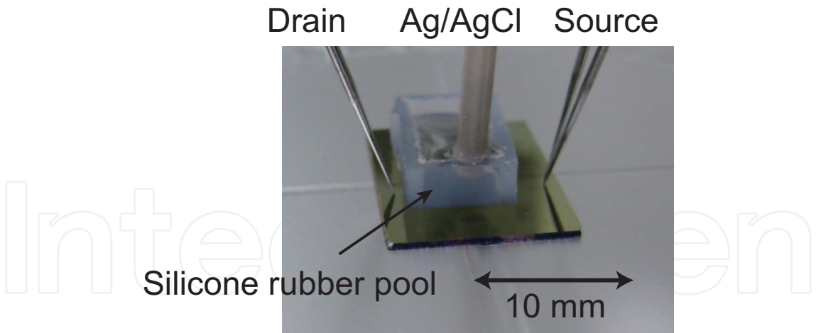
Fig. 4. Photograph of experimental setup with a G-FET.
