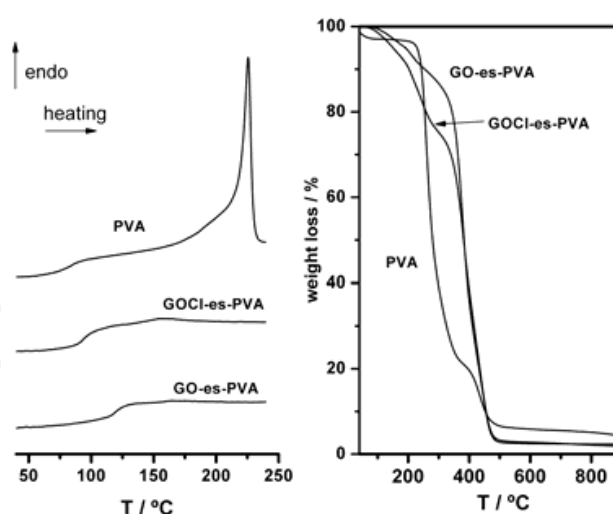
Fig. 11. Thermal behaviour of PVA, and its product of esterification with GO and thionyl chloride treated GO: DSC heating scans at 10\text{ }^\circ\text{C}\cdot\text{min}^{-1} (left) and thermogravimetric curves (right) (Reprinted with permission of The American Chemical Society, 2009).
