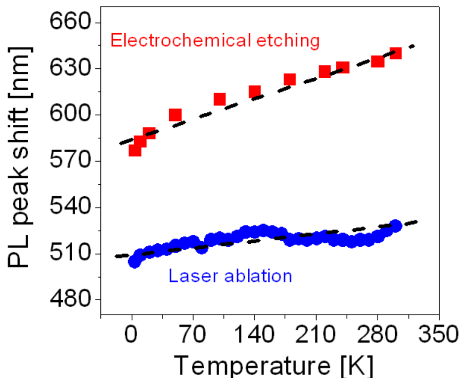
Fig. 2. Shift of PL maxima as a function of temperature for p-type doped Si-ncs prepared by electrochemical etching and laser ablation in water is shown
