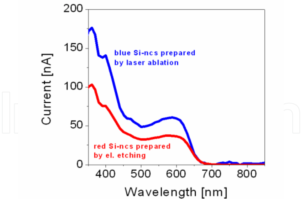
Fig. 8. Photocurrent generation in the Si-ncs/P3HT blends (~38 wt. % concentration of Si-ncs) synthesized by two methods. Red line represents blend with the Si-ncs prepared by electrochemical etching and the blue line by nanosecond laser ablation in water
