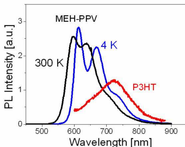
Fig. 5. Photoluminescence (PL) spectra taken at 4 and 300 K of pure MEH-PPV polymer under the same excitation conditions, for comparison. Red line represents typical PL spectrum for P3HT polymer at room temperature
