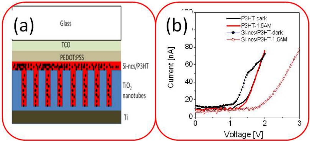
Fig. 11. (a) Schematic sketch of the structure for ordering of Si-ncs/P3HT bulk-heterojunction in TiO 2 nanotube arrays. (b) The current voltage (I-V) characteristics from the pure P3HT polymer and Si-ncs/P3HT blend aligned in within TiO 2 nanotube arrays with the diameters of 90 nm in dark and under illumination AM1.5
