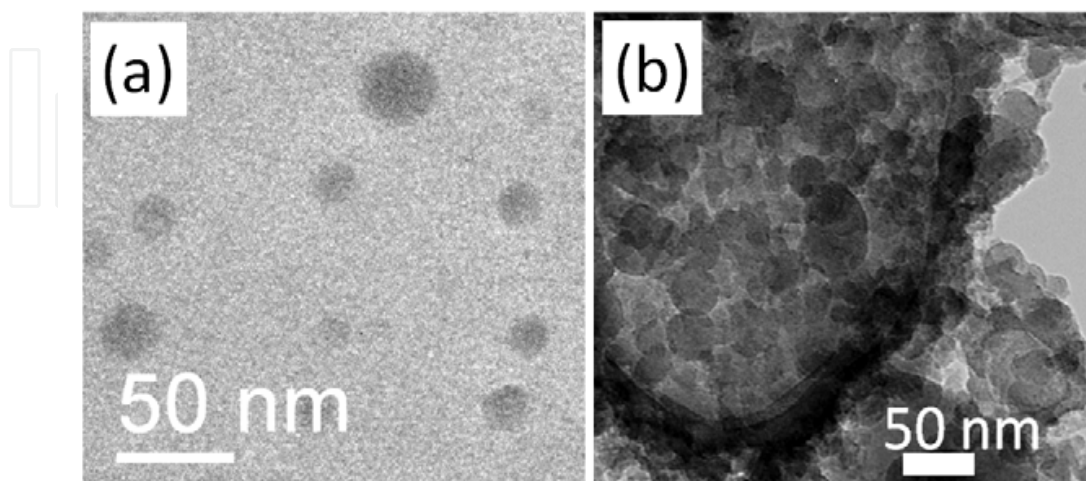
Fig. 4. Transmission electron microscopy (TEM) images of silicon nanocrystals (Si-ncs) prepared (a) by electrochemical etching and (b) by nanosecond excimer KrF laser ablation in water
