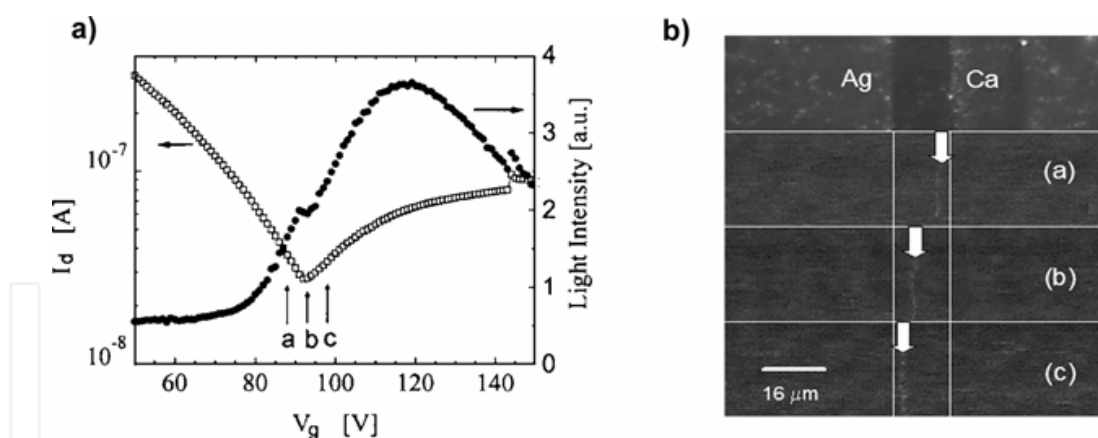
Fig. 5. Transfer characteristic of the SY OLET along with EL intensity (a), image of EL inside the channel at different spatial positions depending on gate bias (b)
