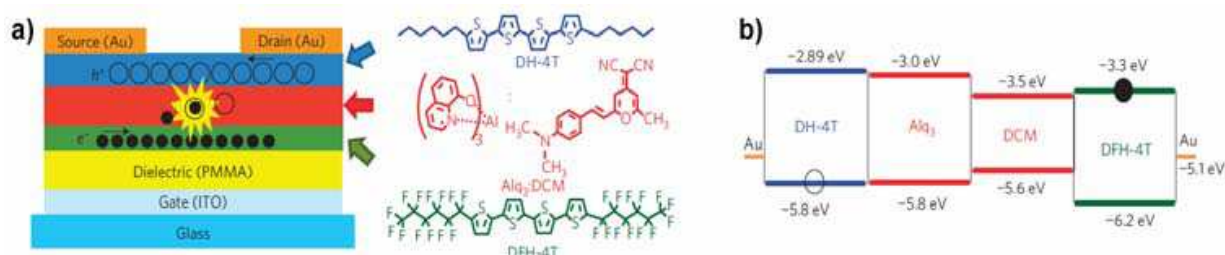
Fig. 10. Tri-layer device structure along with chemical structures of the organic materials used for the device fabrication (a), HOMO and LUMO energetic levels of the materials (b)
